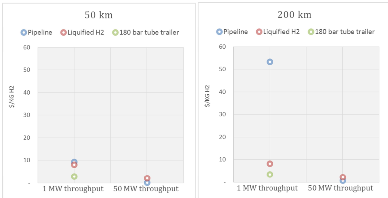
Figure 6: Hydrogen transport pathways comparison (adapted from [3])
