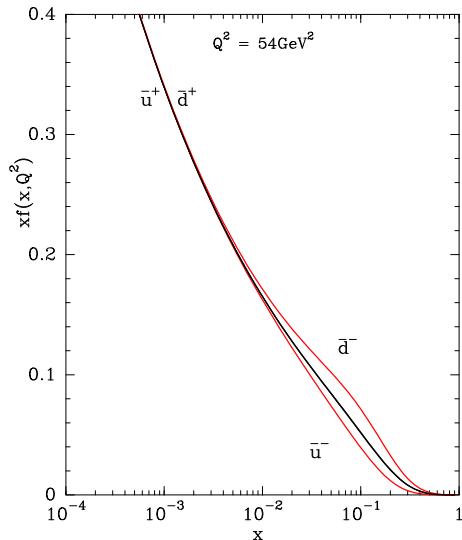
Figure 2: The different helicity components of the light antiquark distributions xf(x, Q^2) ( f = \bar{d}_-, \bar{d}_+ = \bar{u}_+, \bar{u}_- ), versus x , at Q^2 = 54\text{GeV}^2 , after NLO QCD evolution, from the initial scale Q_0^2 = 1\text{GeV}^2 .
