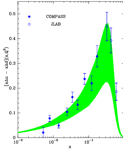
Figure 4: The data on x[\Delta u(x, Q^2) - \Delta d(x, Q^2)] from Refs. [10] (JLab) and [11] (COMPASS), compared to the statistical model prediction at NLO, using Eq. (12) with the corresponding error band.
