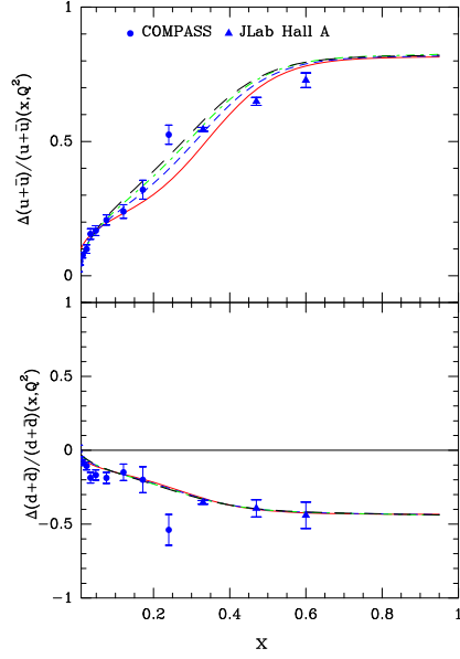
Figure 3: NLO predicted ratios (\Delta u(x, Q^2) + \Delta \bar{u}(x, Q^2)) / (u(x, Q^2) + \bar{u}(x, Q^2)) and (\Delta d(x, Q^2) + \Delta \bar{d}(x, Q^2)) / (d(x, Q^2) + \bar{d}(x, Q^2)) , versus x , at Q^2 (GeV ^2 ) = 1 solid, 10 dashed, 100 dashed-dotted, 1000 long-dashed. Data are from Refs. [10] (Jlab) and [11] (COMPASS).
