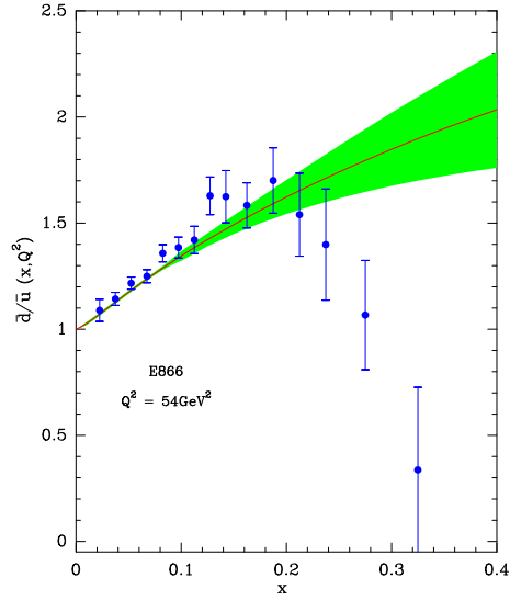
Figure 7: The ratio \bar{d}(x, Q^2)/\bar{u}(x, Q^2) , versus x for Q^2 = 54\text{GeV}^2 . The data from Refs. [7, 8] (E866) are compared with the statistical model prediction with the corresponding error band at NLO.
