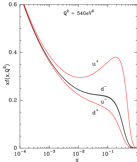
Figure 1: The different helicity components of the light quark distributions xf(x, Q^2) ( f = u_+, u_- = d_-, d_+ ), versus x , at Q^2 = 54\text{GeV}^2 , after NLO QCD evolution, from the initial scale Q_0^2 = 1\text{GeV}^2 .
