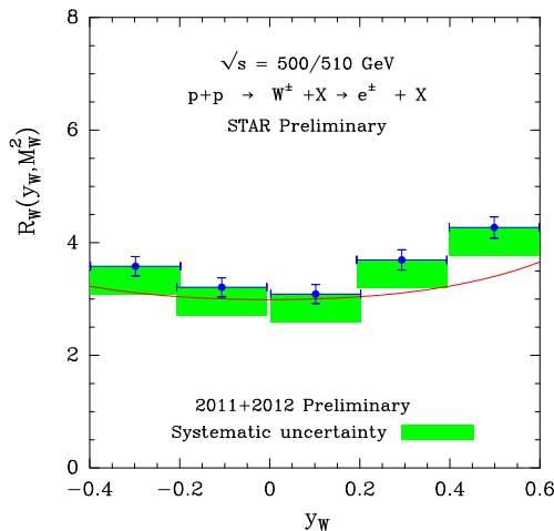
Figure 9: The ratio R_W = W^+/W^- , versus the W rapidity y_W for Q^2 = M_W^2 \text{ GeV}^2 \sqrt{s} = 500/510 GeV calculated at NLO. Preliminary data are from Ref. [20]
