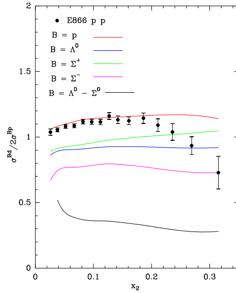
Figure 8: The Drell-Yan cross section ratios of \sigma(Bd)/2\sigma(Bp) versus x_2 (momentum fraction of the target partons) data from (E866) Refs. [7, 8]. The curves are the statistical model predictions for different incoming beams B = p, \Lambda^0, \Sigma^+, \Sigma^-, \Lambda^0 - \Sigma^0 at p_{lab} = 800\text{GeV} .
