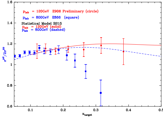
Figure 6: The Drell-Yan cross section ratios of \sigma(pd)/2\sigma(pp) versus x_{target} (momentum fraction of the target partons) data from (E866) p_{lab} = 800 GeV Refs. [7, 8], SeaQuest E906 p_{lab} = 120 GeV . The curves are the statistical model predictions at NLO.
