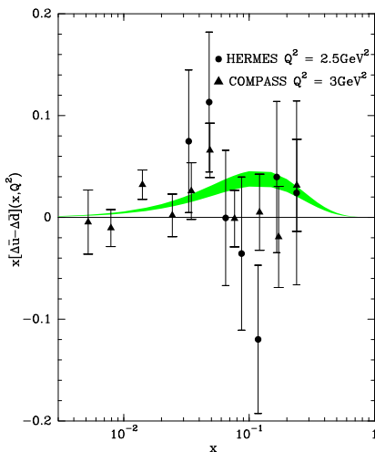
Figure 5: The data on x[\Delta\bar{u}(x, Q^2) - \Delta\bar{d}(x, Q^2)] from Refs. [14] (HERMES) and [11] (COMPASS), compared to the statistical model prediction at NLO, using Eq. (13) with the corresponding error band.
