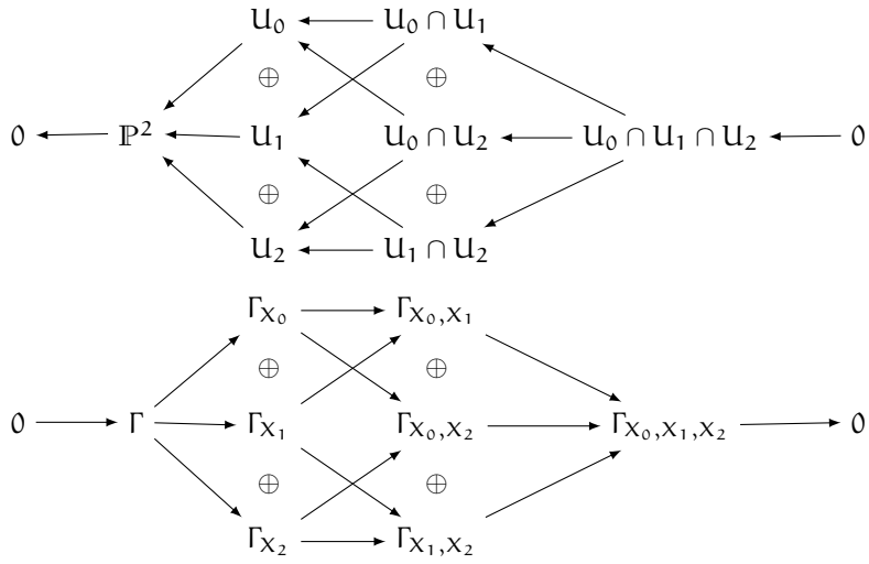
Figure 1: Čech Complex for \mathbb{P}_K^{n, \text{ad}, \text{perf}} , n = 2
