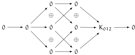
Figure 2: 3 negative exponents
