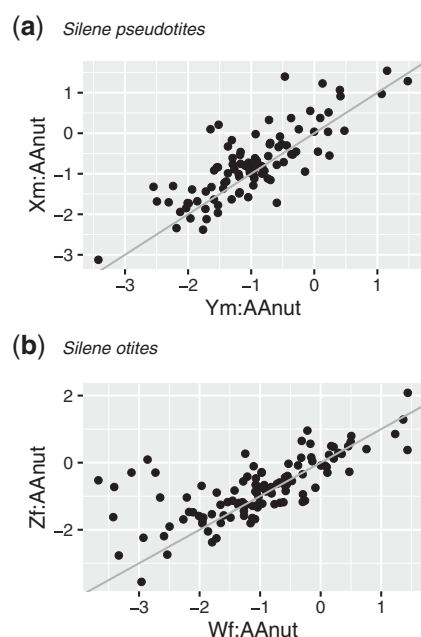
FIG. 2. —Correlation between the expression of X (or Z) and Y (or W) in the heterogametic sex for (a) S. pseudotites and (b) S. otites . Xm = male X allele expression, Ym = male Y allele expression, Zf = female Z allele expression, Wf = female W allele expression, and AAut = genotype expression of orthologs in the nondioecious S. nutans that do not have sex chromosomes (therefore, orthologs are on autosomes). Diagonal lines across the plot show no change in expression.
