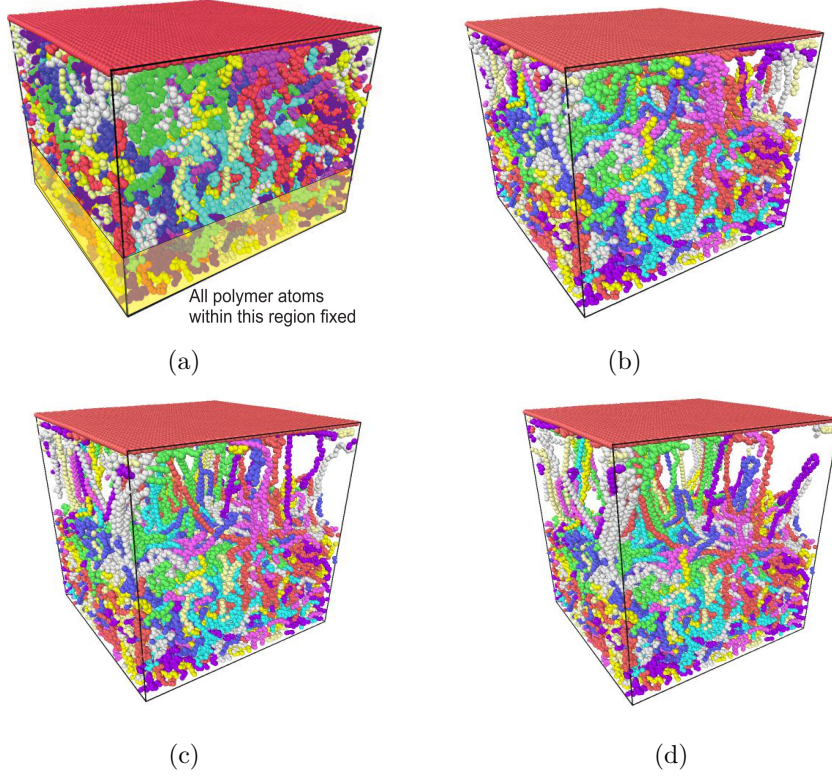
Figure 2. Evolution of the atomistic model during the normal separation. The model contains 44860 atoms, and the graphene is moved with a step of 0.5 Å. The graphene atoms and the bottom layer of the polymer are fixed during the relaxation.
