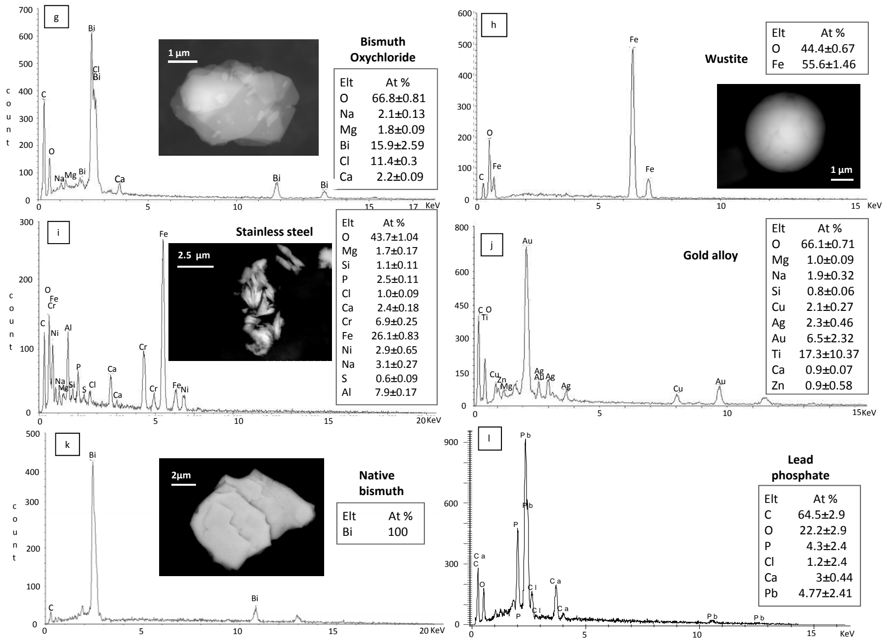
Figure 2: Electron micrographs and EDXS spectra of typical heavy metal-bearing particles found in Golden Star urban effluent.
