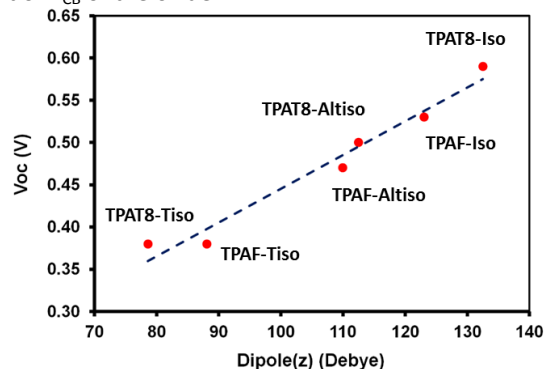
Figure 9: Open-circuit voltage variation as a function of the dipole of the of the oxidized dyes
