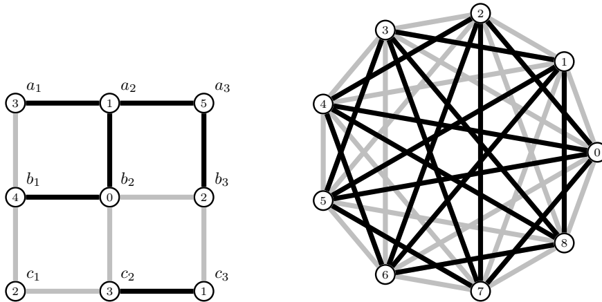
Figure 4: A 2-edge-coloured 6-colouring of a signature of G(3,3) (left), and the 2-edge-coloured circulant graph C(9, \{2,4\}) (right). Black (resp. gray) edges are positive (resp. negative) edges.
