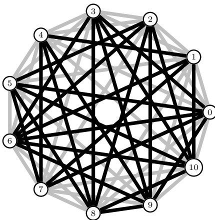
Figure 1: The 2-edge-coloured graph A_{11} . Black (resp. gray) edges are positive (resp. negative) edges.
