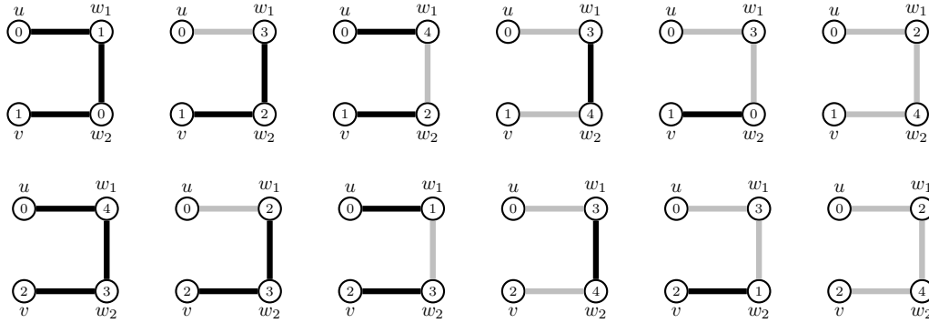
Figure 3: Examples of the 2-edge-coloured 3-paths of C(5, \{1\}) claimed in the proof of Observation 4.4, for (u, v) = (0, 1) (top), and (u, v) = (0, 2) (bottom). Black (resp. gray) edges are positive (resp. negative) edges.
