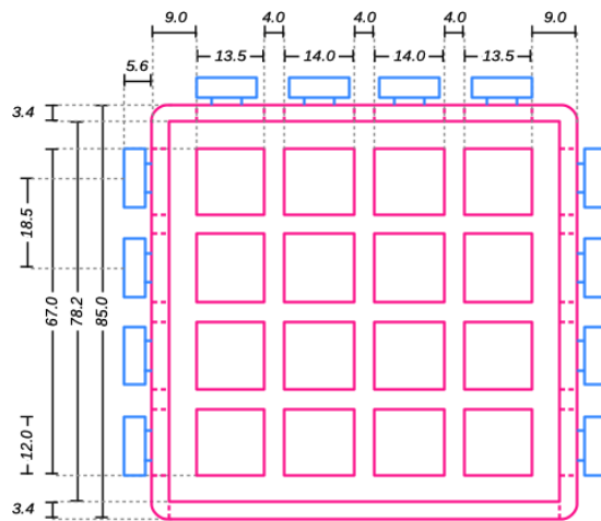
Figure 3: Prototype size.
