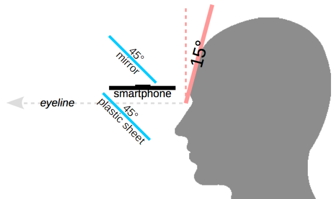
Figure 3. Pepper's ghost configuration and forehead slope
