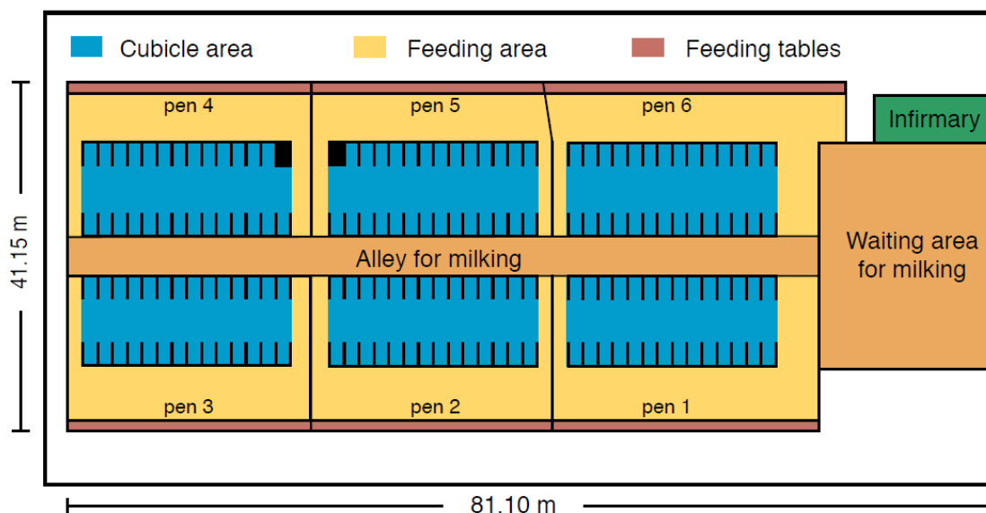
Figure 1: Barn composed of 6 pens, each with a capacity of accommodating 28 cows.
