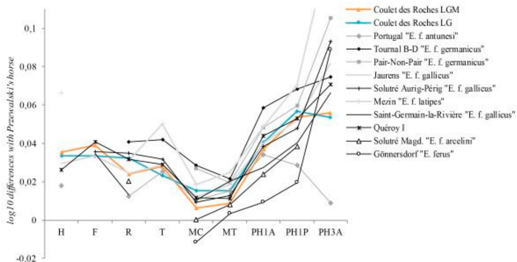
Figure 22. Ratio diagram of bone length and third phalanx breadth of Pleistocene horses. Coulet des Roches measurements in Table 13. Reference: Przewalski’s horse [79]. Comparative data: Jaurens and Mezin [79]; Portugal [80]; Tournal B-D [81]; Gönnersdorf [86]; Pair-non-Pair, Saint-Germain-la-Rivière [88]; Solutré [89]; Quéroy I [82]. Abbreviations: H, Humerus; F, Femur; R, Radius; T, Tibia; MC, Metacarpal; MT, Metatarsal; PH1A, First Anterior Phalanx; PH1P, First Posterior Phalanx; PH3A, Third Anterior Phalanx.
