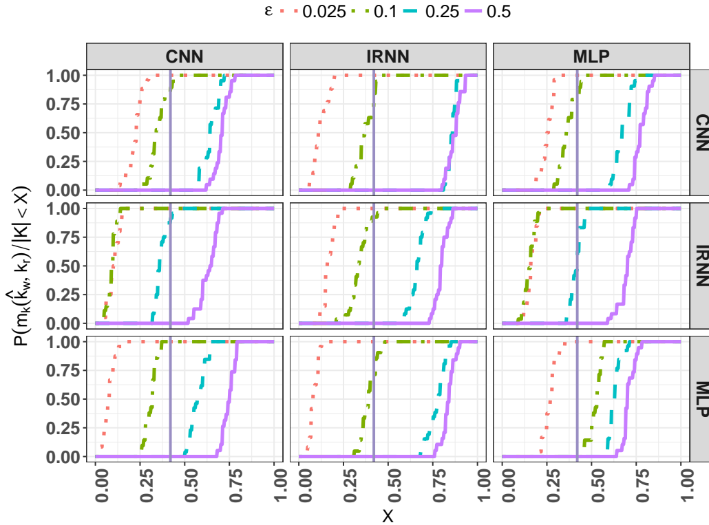
Fig. 6 Distribution of (normalized) Hamming distance when extracting the watermark (generated on networks k_w listed on right axis) from remote unmarked models k_r (w. names on the top), for |K| = 100 and four values of \varepsilon . Vertical solid bars indicate the decision threshold corresponding to p < .05 criteria. False positives ( i.e. , unmarked model at distance less than the threshold) happen when the CDF is on the left of the bar. Algorithm 1’s value \varepsilon = 0.5 (purple solid curve) prevents the issue of false positives in all cases.
