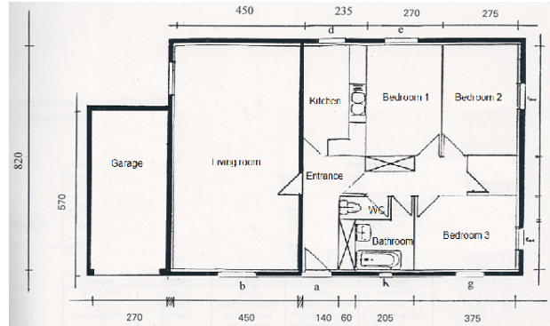
Figure 8: The tested residential building, MOZART
