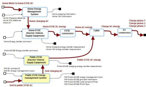
Figure 10: Charging spot organic architecture
