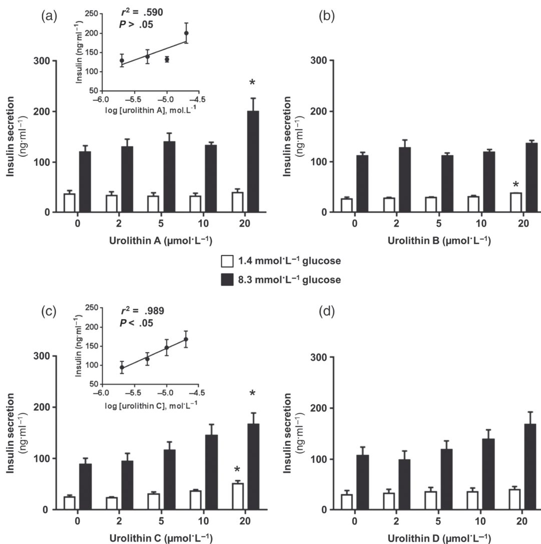
FIGURE 1 Effects of urolithins A, B, C, and D on basal and glucose-induced insulin secretion in INS-1 cells. The effects of increasing concentrations ( 2\text{--}20 \mu\text{mol}\cdot\text{L}^{-1} ) of (a) urolithin A, (b) urolithin B, (c) urolithin C, and (d) urolithin D in INS-1 cells were determined under basal non-stimulating ( 1.4 \text{ mmol}\cdot\text{L}^{-1} glucose) or 8.3 \text{ mmol}\cdot\text{L}^{-1} glucose-stimulated conditions. Inserts depict the correlation between insulin secretion and the log of urolithin concentration. Under non-stimulating glucose condition, there was a significant effect of the treatment for urolithin B and C. Under 8.3 \text{ mmol}\cdot\text{L}^{-1} glucose-stimulated condition, there was a significant effect of the treatment for urolithins A and C. * P < .05 , significantly different from 0 \mu\text{mol}\cdot\text{L}^{-1} urolithin, one-way ANOVA with Holm–Sidak test, n = 5
