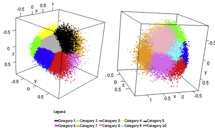
Fig. 2. Classification in 10 categories according to the first 3 dimensions (1,2,3).
