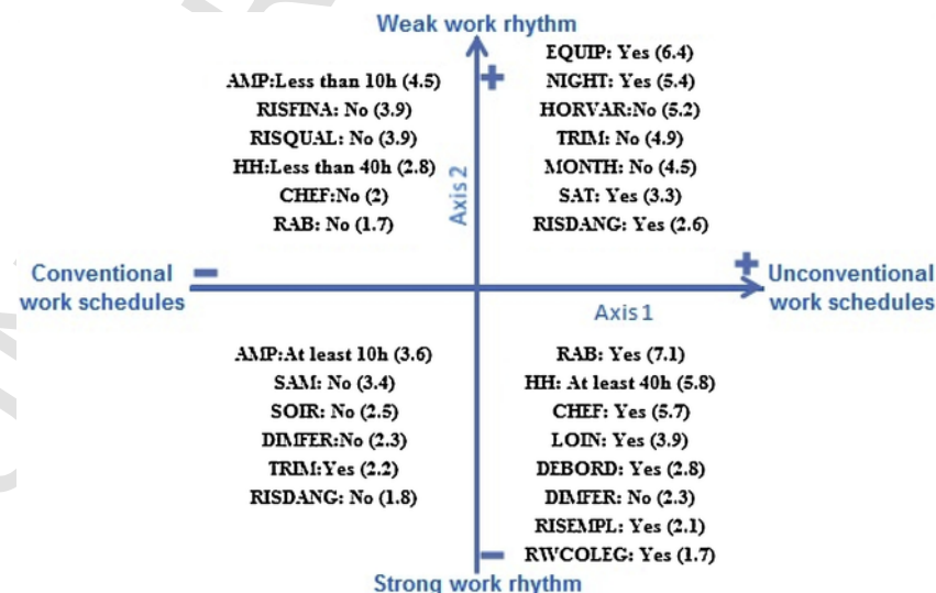
Fig. 1. Active representative modalities and their contributions (in brackets) on the factorial plane (axis 1, axis 2).
