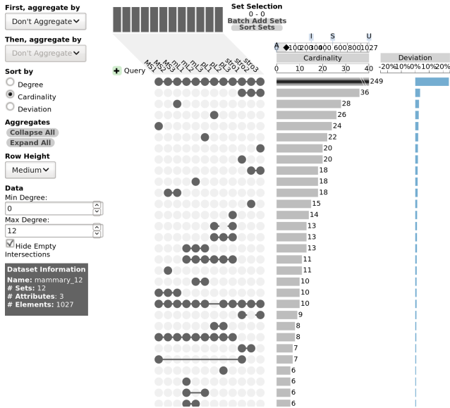
Fig. 11. UpSet displaying the mammary tissue dataset.
