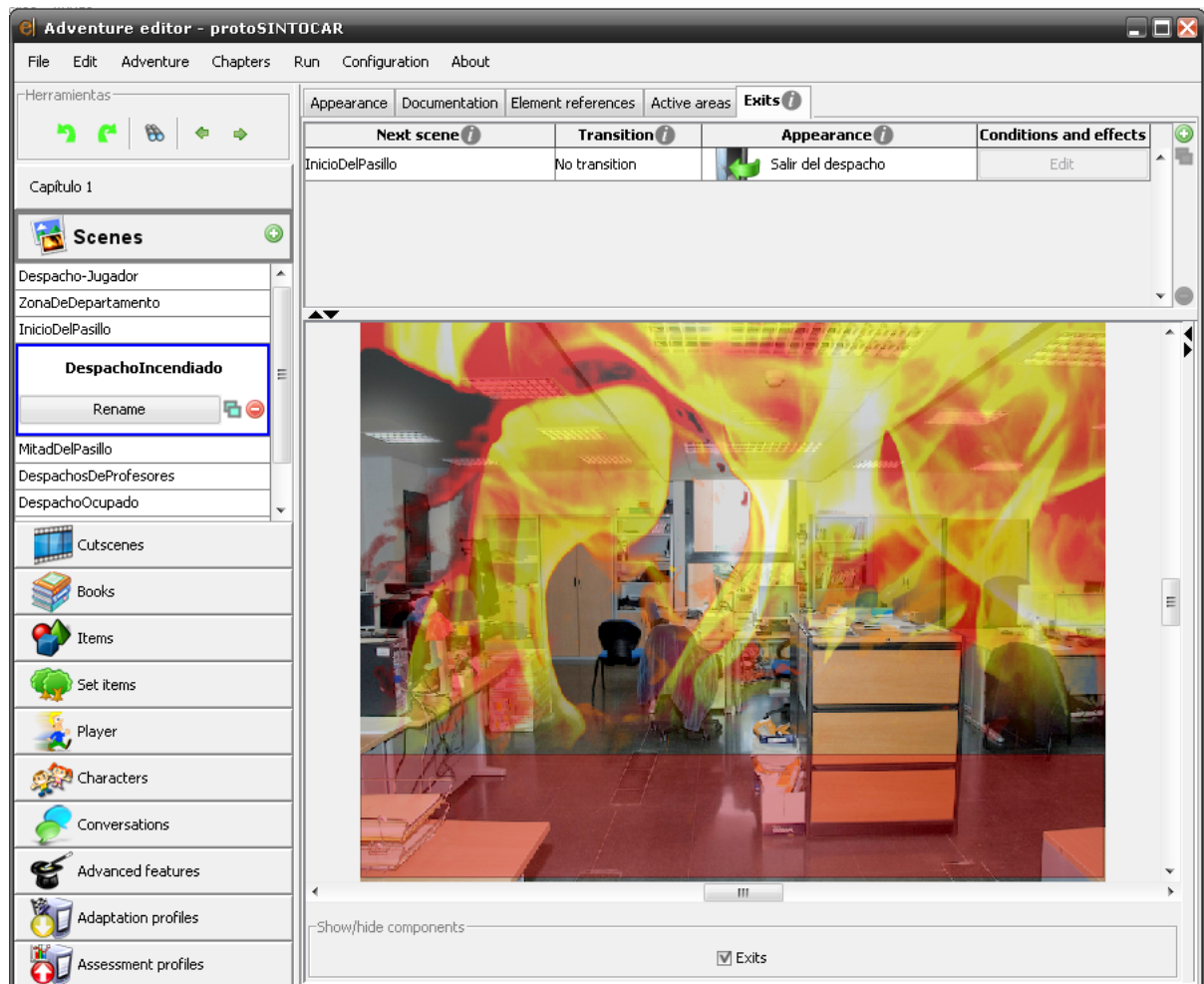
Fig. 5 e-Aventure, an editor to create serious adventure games (source: e-adventure.e-ucm.es)
