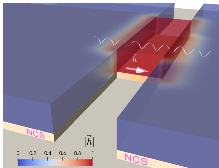
Figure 1. The Chiral Magnetic Josephson junction: two non-centrosymmetric superconductors (NCSs) are weakly linked by a uniaxial ferromagnet (F). The exchange field \mathbf{h} of the ferromagnet, oriented across the link, induces an inversion symmetry-breaking component of the supercurrent (represented by the spiral) in the junction.
