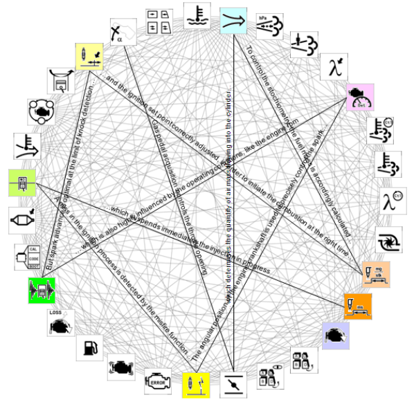
Figure 3. Representation of some functional aggregates, and their relationships. The software link, visible as data or control flow between the components is a consequence of the physical interaction between the controlled system actuators via the physical processes of the controlled system.
