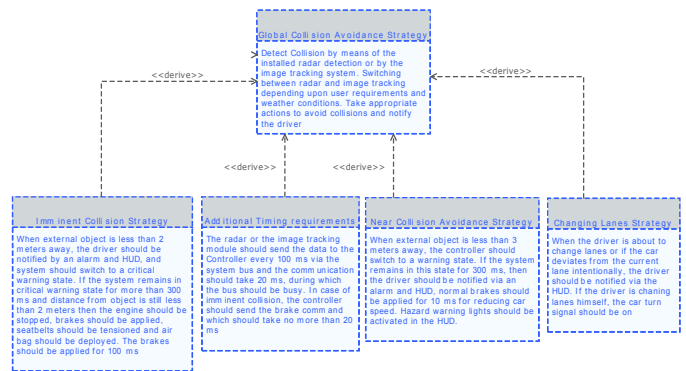
Figure.4: Initial requirements specifications for the CCAS
