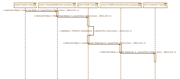
Figure.23: Sequence SendSensorDistanceToCtrl for radar/controller communication
