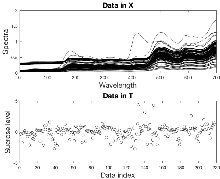
Fig. 4: The orange juice dataset. The upper panel shows the high-dimensional data ( X ) and the lower one shows the low-dimensional data ( T ).
