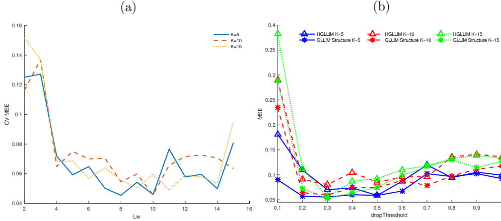
Fig. 5: Results for the user-defined parameters of the orange juice dataset. (a) The HGLLiM cross-validation results for different K and L_w . (b) The prediction MSE of different K and different methods against different dropThreshold .
