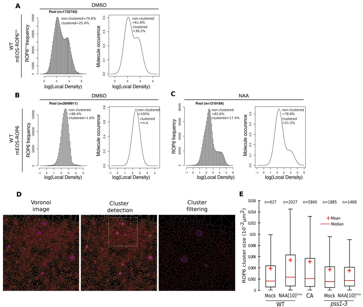
Figure S6. Raw data of live PALM experiments presented in the paper. A-C, Left panels represent the frequency of mEos-ROP6 and mEos-ROP6 CA molecules according to their local density (log(local density)) obtained by analysing tessellation-based automatic segmentation of super-resolution images in mock and auxin-treated condition (NAA, 10 \mu M, 5min) in WT. Right panel represents the distribution of mEos-ROP6 and mEos-ROP6 CA according to their local density (log(local density)) obtained by analysing the frequency plot (left panel) using the R mClust package. The percentage of low and high local density in each graph represents the percentage of molecules below and above the log(local density) of 3.5, respectively. Note that the percentage in left and right panels for each condition are similar (i.e. they vary only from few percent), confirming the existence of two populations with a normal distribution. Note that the right plots in B and C are similar to the plot in Fig. 3G. “n” corresponds to the number of molecules analysed. D , Example of Voronoi images obtained after extracting local density from tessellation-based automatic segmentation of super-resolution images (left image), cluster detection and filtering of local density (middle image, zoom in right image) in the Voronoi image and E , quantification of the respective size of the cluster in (from left to right), mEos-ROP6 mock-treated, mEos-ROP6 NAA-treated (5min, 10 \mu M), mEos-ROP6 CA mock-treated, mEos-ROP6 mock-treated in pss1-3 and mEos-ROP6 NAA-treated in pss1-3 (5min, 10 \mu M). “n” corresponds to the number of nanocluster analysed.
