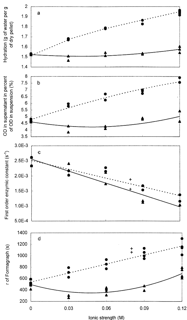
Fig. 2. Physicochemical changes obtained on dispersion of casein micelles in salt solutions of increased ionic strength. (---●---), NaCl; (—▲—), CaCl 2 ; (+), milk ultrafiltrate (a) Pellet hydration versus ionic strength. (b) Optical density (OD) in supernatant in percent of total OD. (c) First-order enzymic constant. (d) r , the clotting time from formagraph.
