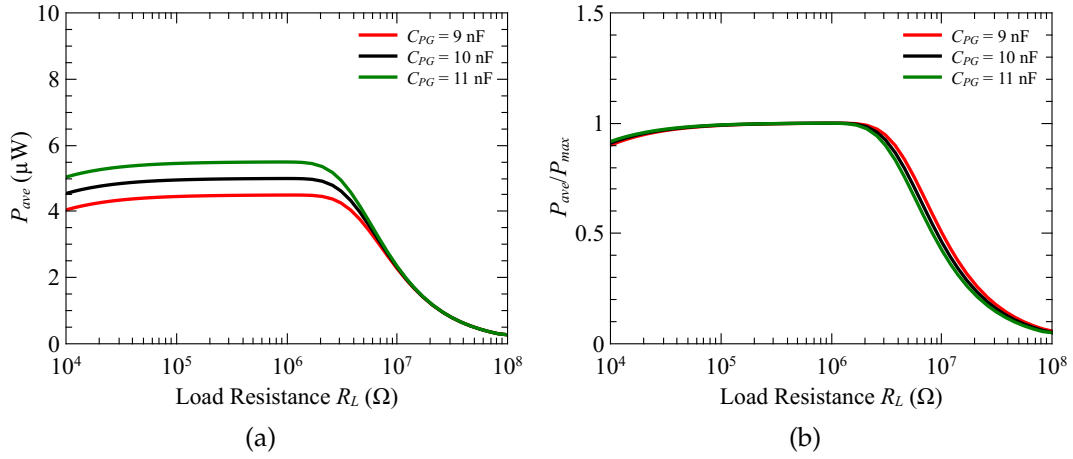
Figure 11: Computed average power (a) and normalized computed mean power according to the max value (b) as a function of the load R_L , for different values of the internal capacitance for a exponential waveform with a \tau/T = 5 \times 10^{-5} .
