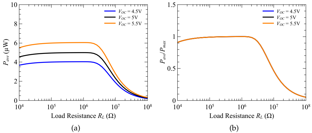
Figure 12: Computed average power (a) and normalized computed mean power according to the max value (b) as a function of the load R_L , for different values of the open circuit voltage for a exponential waveform with a \tau/T = 5 \times 10^{-5} .
