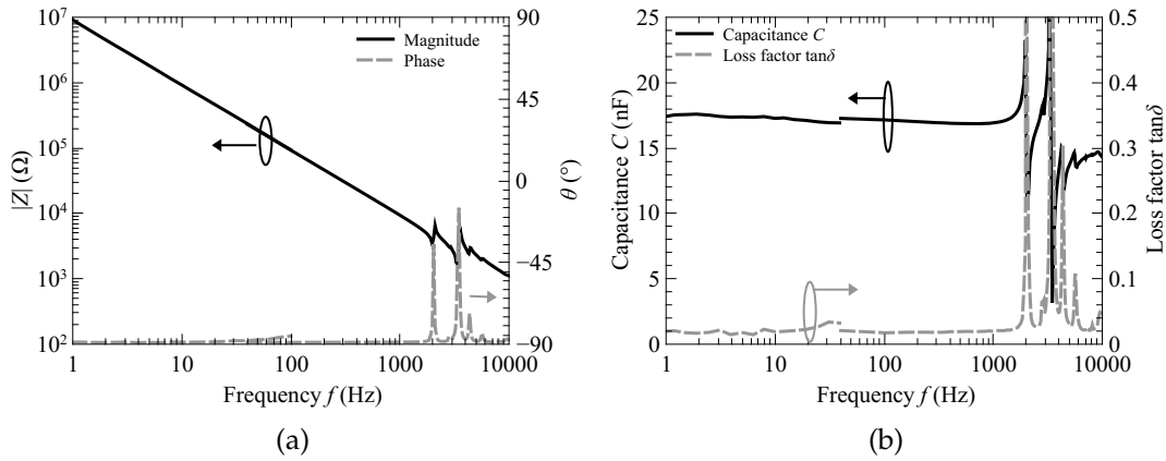
Figure 15: Magnitude and phase of the impedance (a) and associated capacitance and loss factor (b) of the piezoelectric buzzer as a function of frequency.
