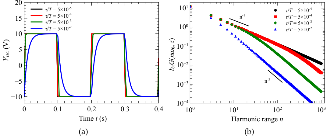
Figure 7: Waveform of the periodic exponential signal (a) and the corresponding harmonic content (b) for different values of \tau/T . Only odd coefficients are represented since even coefficients are null.
