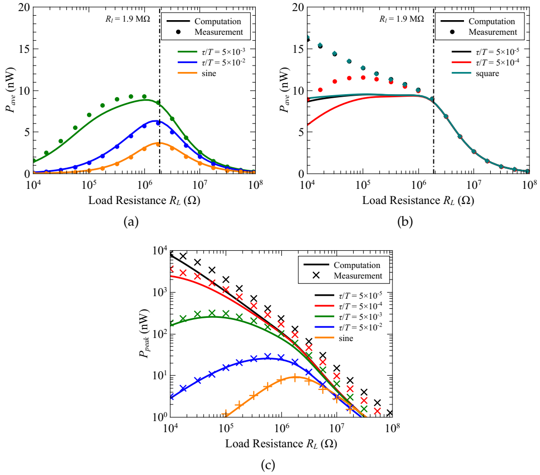
Figure 16: Measured average power (a), (b) and peak power (c) for the PZT buzzer compressed by a NAC2015 actuator, for different values of \tau/T . The curves for an exponential signal with \tau/T = 5 \times 10^{-5} and for the square signal are superimposed.
