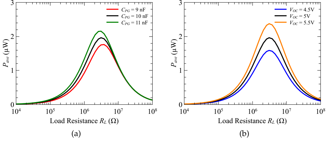
Figure 10: Computed average power as a function of the load R_L , for different values of the internal capacitance (a) and different values of the open circuit voltage (b).
