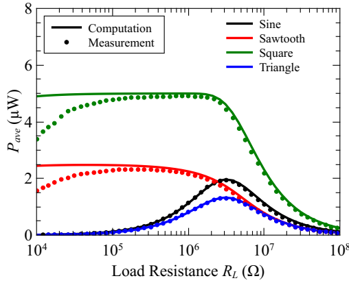
Figure 4: Computed (lines) and measured (bullets) mean power supplied to the load as a function of the load R_L for different waveforms.
