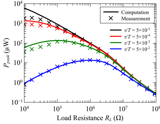
Figure 9: Measured (cross) and computed (lines) peak instantaneous powers for different values of \tau/T , for an exponential waveform.
