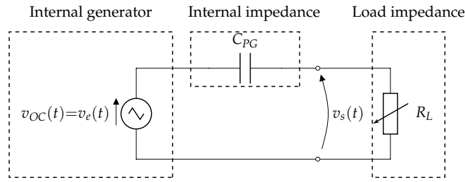
Figure 3: Equivalent circuit of the PG presenting a capacitive impedance, and connected to a resistive load for the experimental tests.
