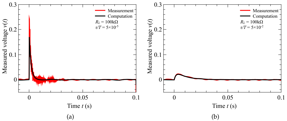
Figure 17: Measured and computed waveform for R_L = 100 k \Omega , for an exponential signal with \tau/T = 5 \times 10^{-5} (a) and \tau/T = 5 \times 10^{-2} (b).
