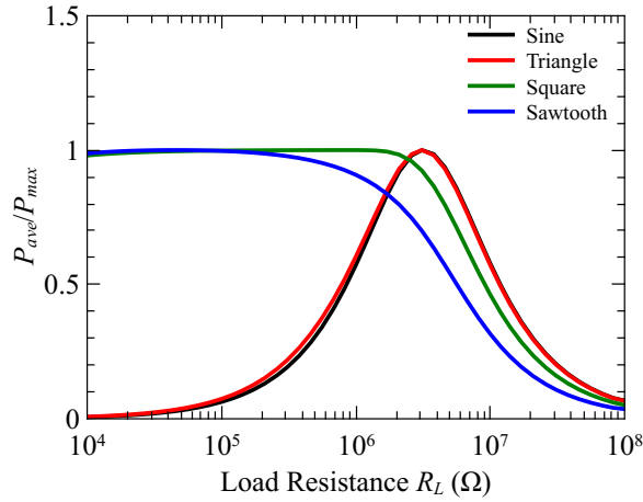
Figure 5: Normalized computed mean power according to the max value as a function of the load R_L for different waveforms.
