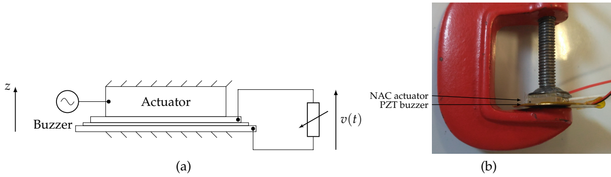
Figure 13: Schematic (a) and optical view (b) of the experimental test bench using a piezoelectric actuator and a piezoelectric buzzer (the PG). The actuator and the buzzer are fixed together using a small screw. The force is applied across the z -axis.
