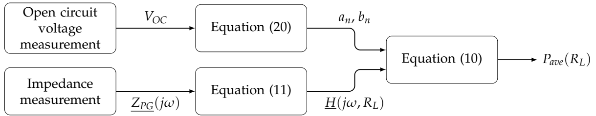
Figure 14: Workflow used to compute the average power as a function of the resistive load using the open circuit measurement and the impedance measurement.
