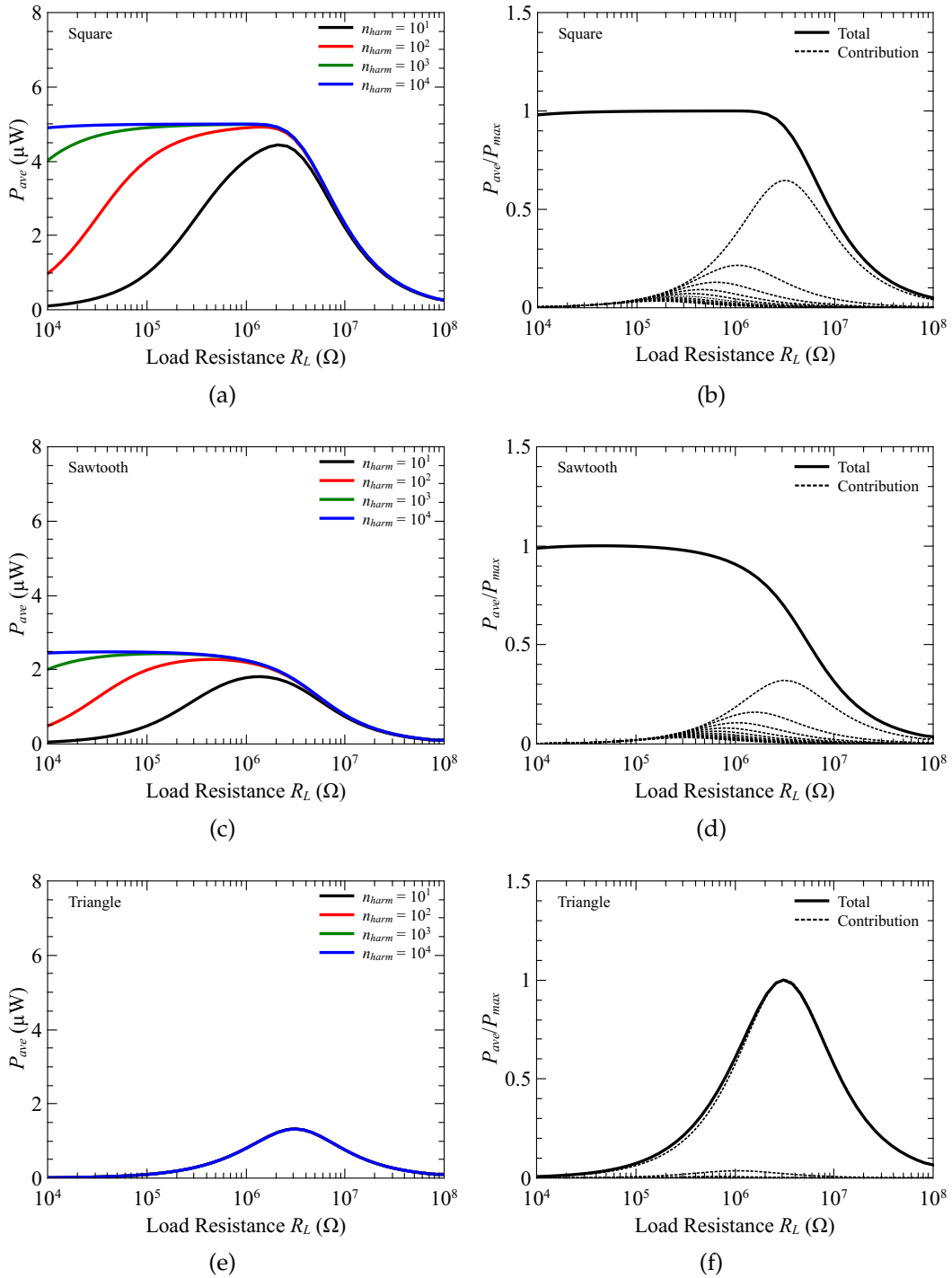
Figure 6: Mean power as a function of the load R_L for increasing number of harmonics used for the computation, when V_{OC} is a square signal (a), a sawtooth signal (c) or a triangle signal (e). Decomposition (dashed line) and total (full line) power as a function of the load R_L , when V_{OC} is a square signal (b), a sawtooth signal (d) or a triangle signal (f).
