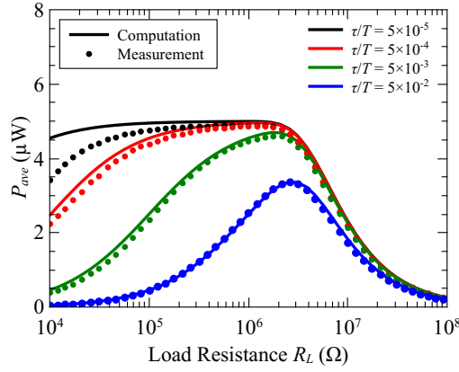
Figure 8: Measured (bullets) and computed (lines) power as a function of the load, for the periodic exponential signal having different values of \tau/T .
