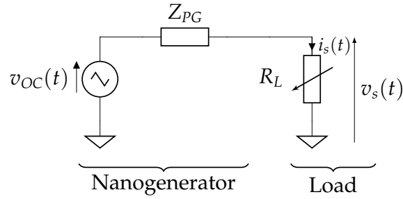
Figure 1: Common electrical circuit used for functional characterization of PGs.
