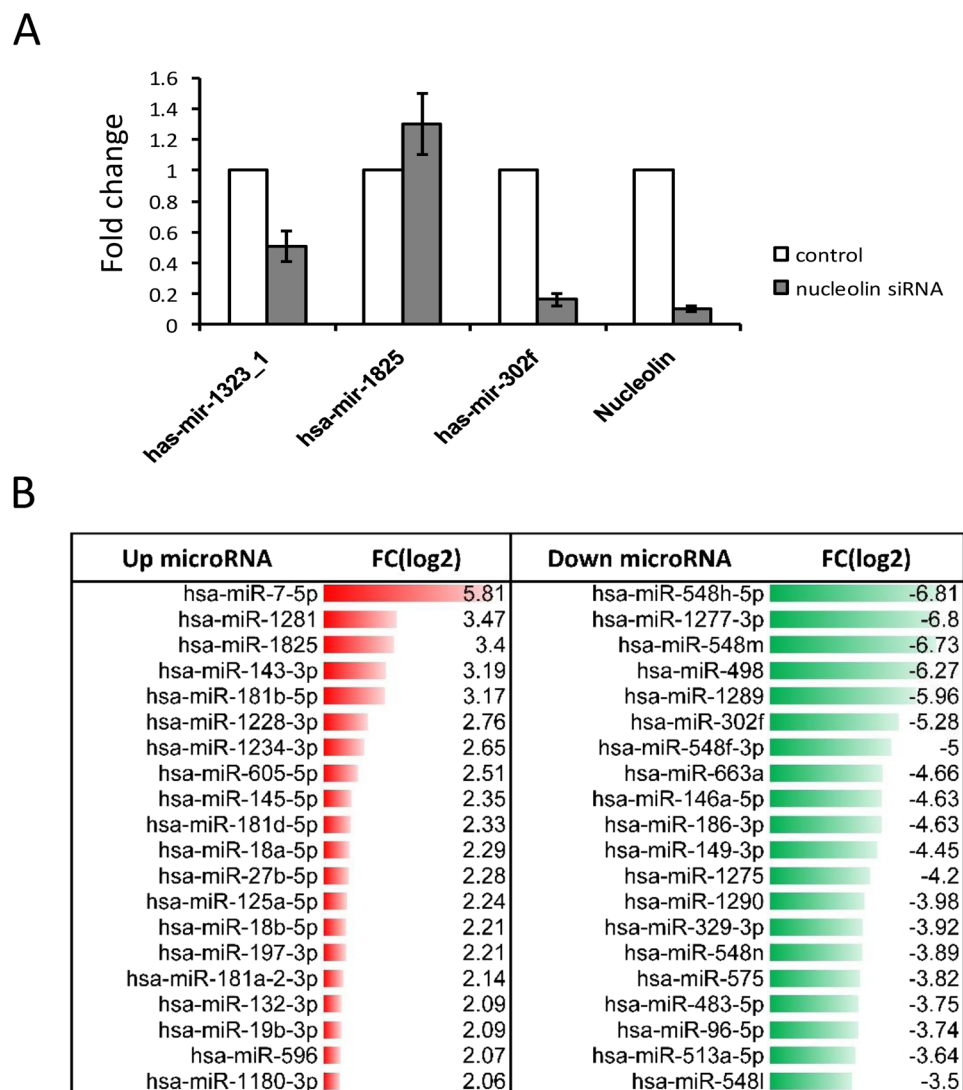
Figure 7. miRNAs expression analysis in NCL depleted HeLa cells. (A) Fold change of randomly selected miRNAs (Upregulated Hsa-miR-1825 and down regulated hsa-miR-1323 -hsa-miR-302f and NCL) as determined by RT-qPCR. (B) First 20 differentially expressed (Up/Down) microRNAs with FC \geq \pm 1.5 and p-value \leq 0.05 .
