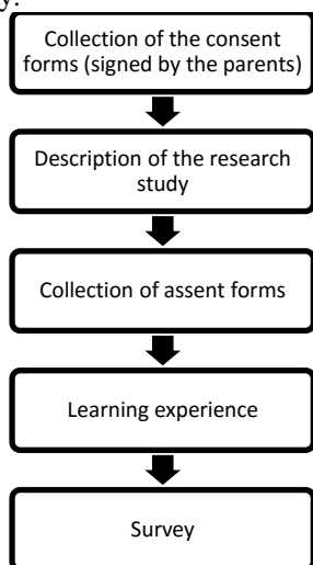
Figure 7: Evaluation process.
