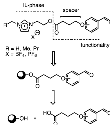
Figure 1. Grafted ionic liquid phases for liquid-phase organic synthesis (LPOS).
