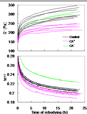
Fig.1. Short-term rebodding: viscoelastic properties for 20 h after stirring
