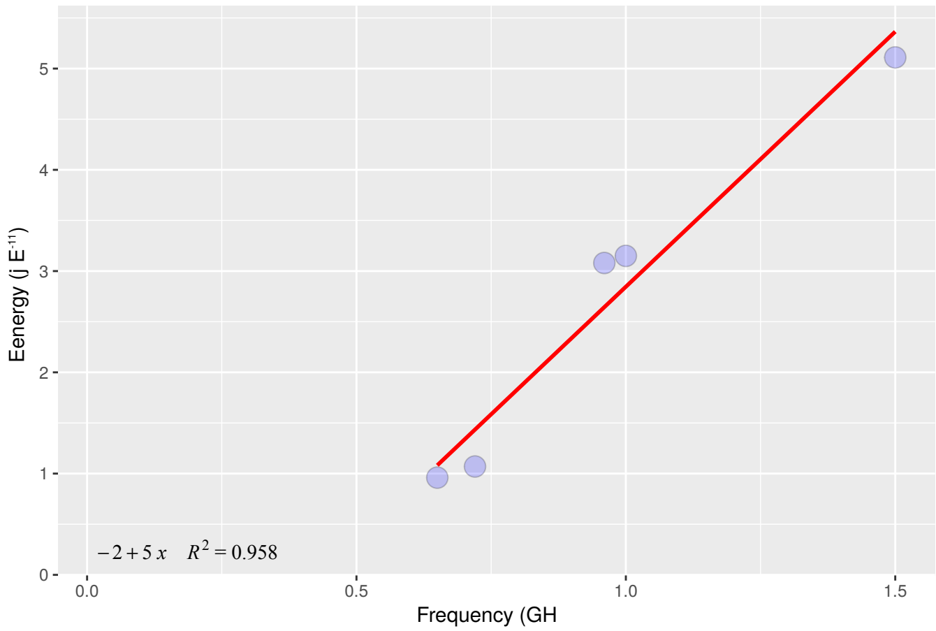
Figure 9 Dynamic energy dissipated by clock cycle in function of the frequency for the RVFF scenario
