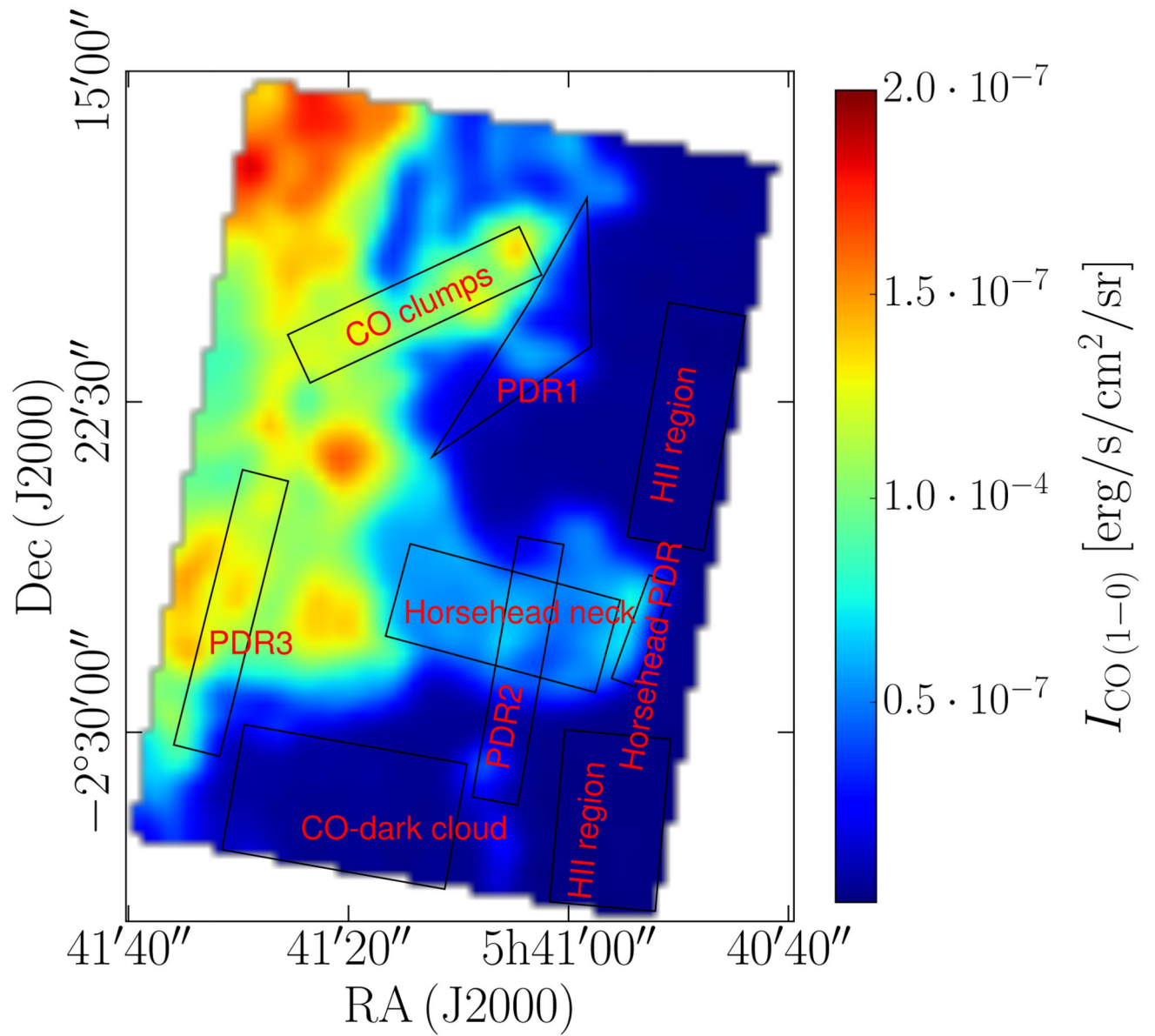
Fig. 3. CO(1-0) line-integrated intensity convolved to 36'' resolution with selected regions (see Sec. 3.2) indicated.
