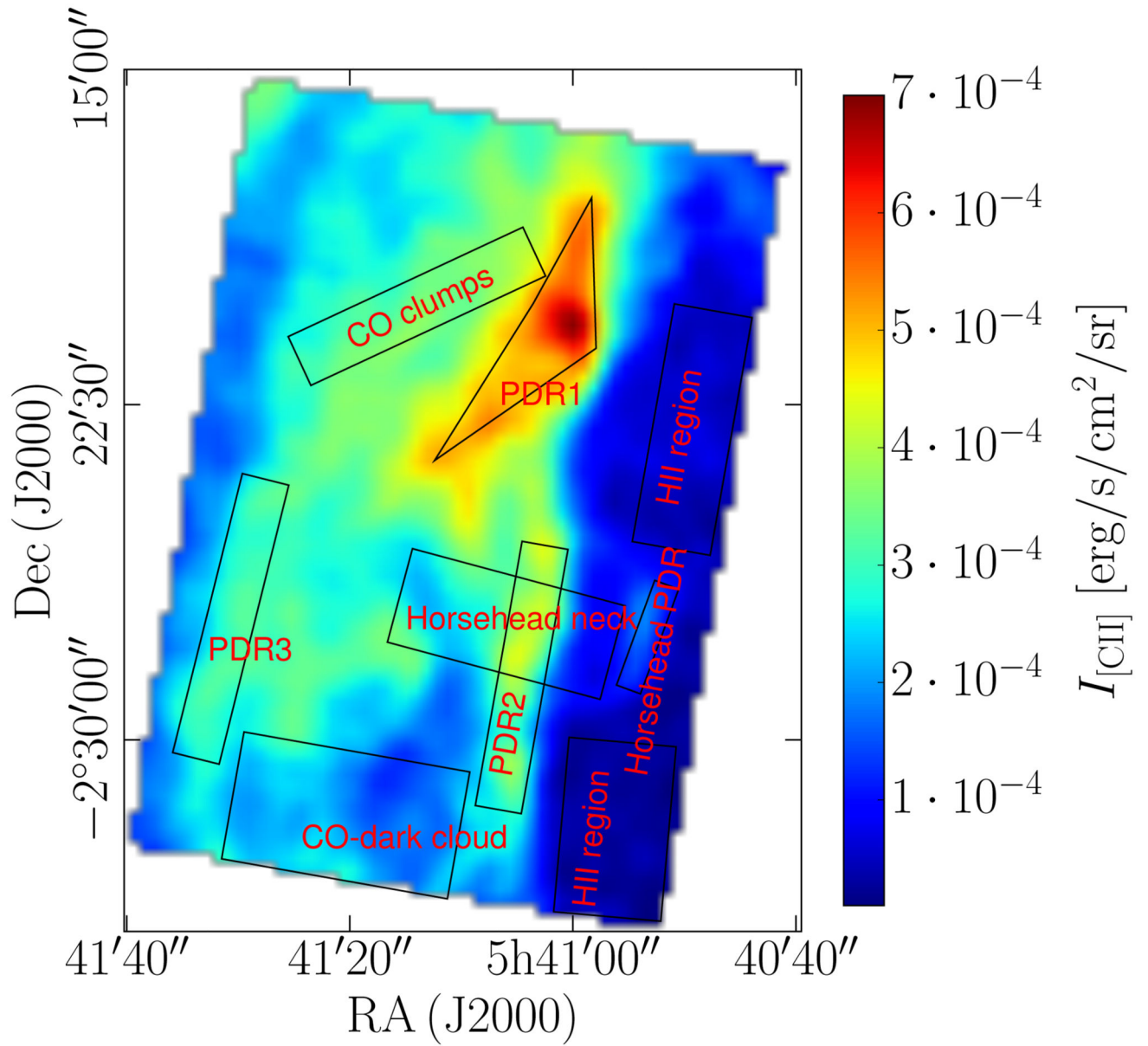
Fig. 2. [CII] line-integrated intensity convolved to 36'' resolution with selected regions (see Sec. 3.2) indicated.
