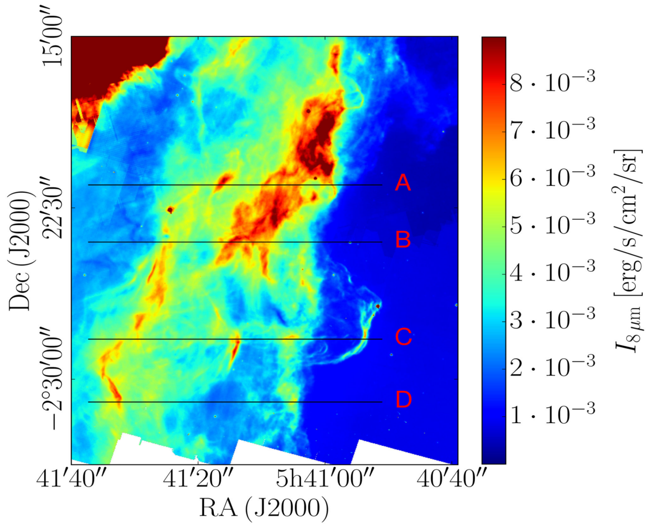
Fig. 15. IRAC 8\ \mu\text{m} image with lines A, B, C, and D indicated.
