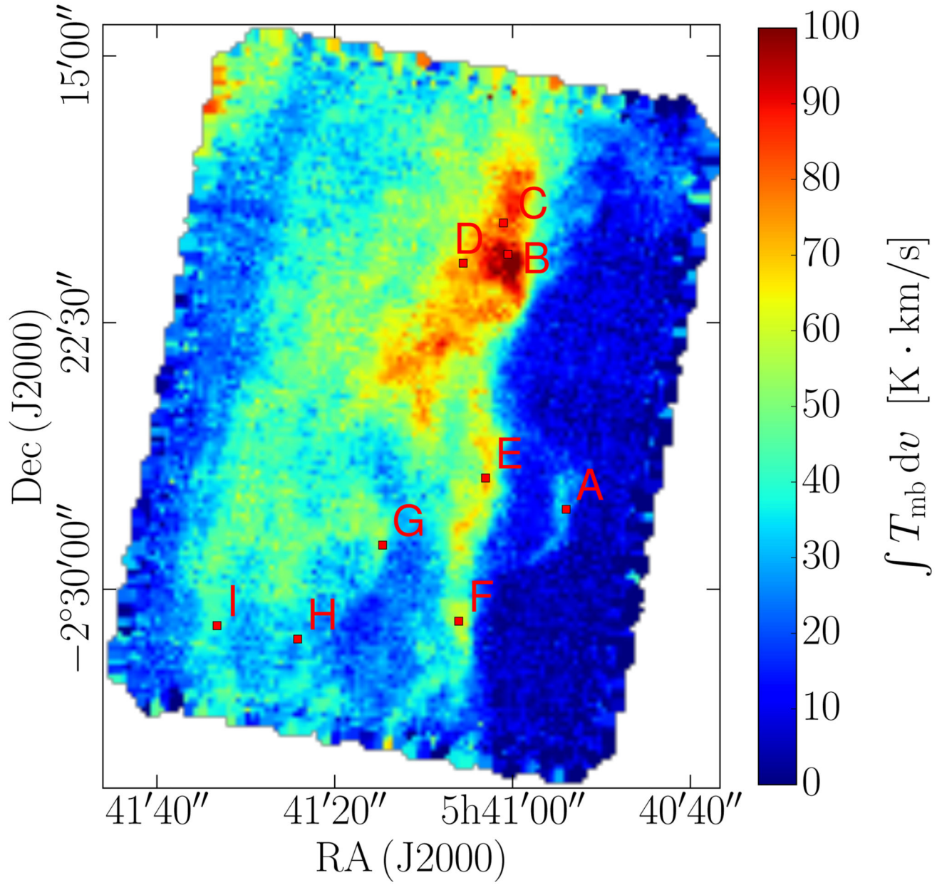
Fig. 1. [Cu II] line-integrated intensity; points indicate positions where individual spectra are extracted for illustrative purposes (see Sec. 3.3).
