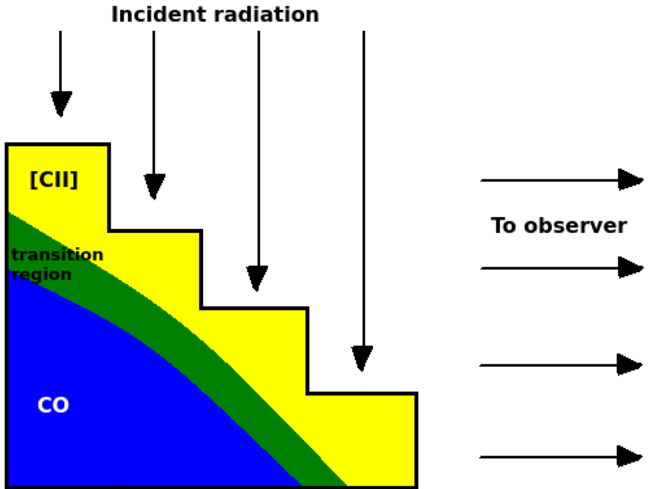
Fig. 17. Geometry of the L1630 molecular cloud surface
