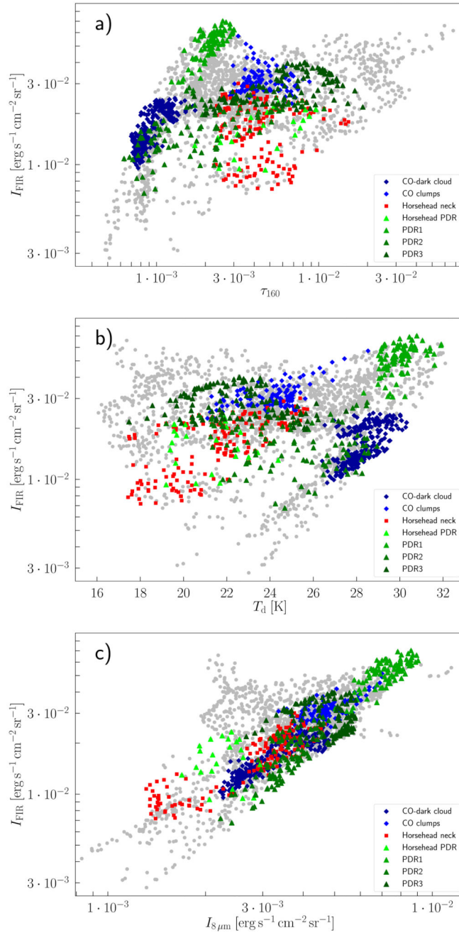
Fig. 11. Correlation plots of I_{\text{FIR}} versus \tau_{160} , T_{\text{d}} , and I_{8\ \mu\text{m}} , respectively.
