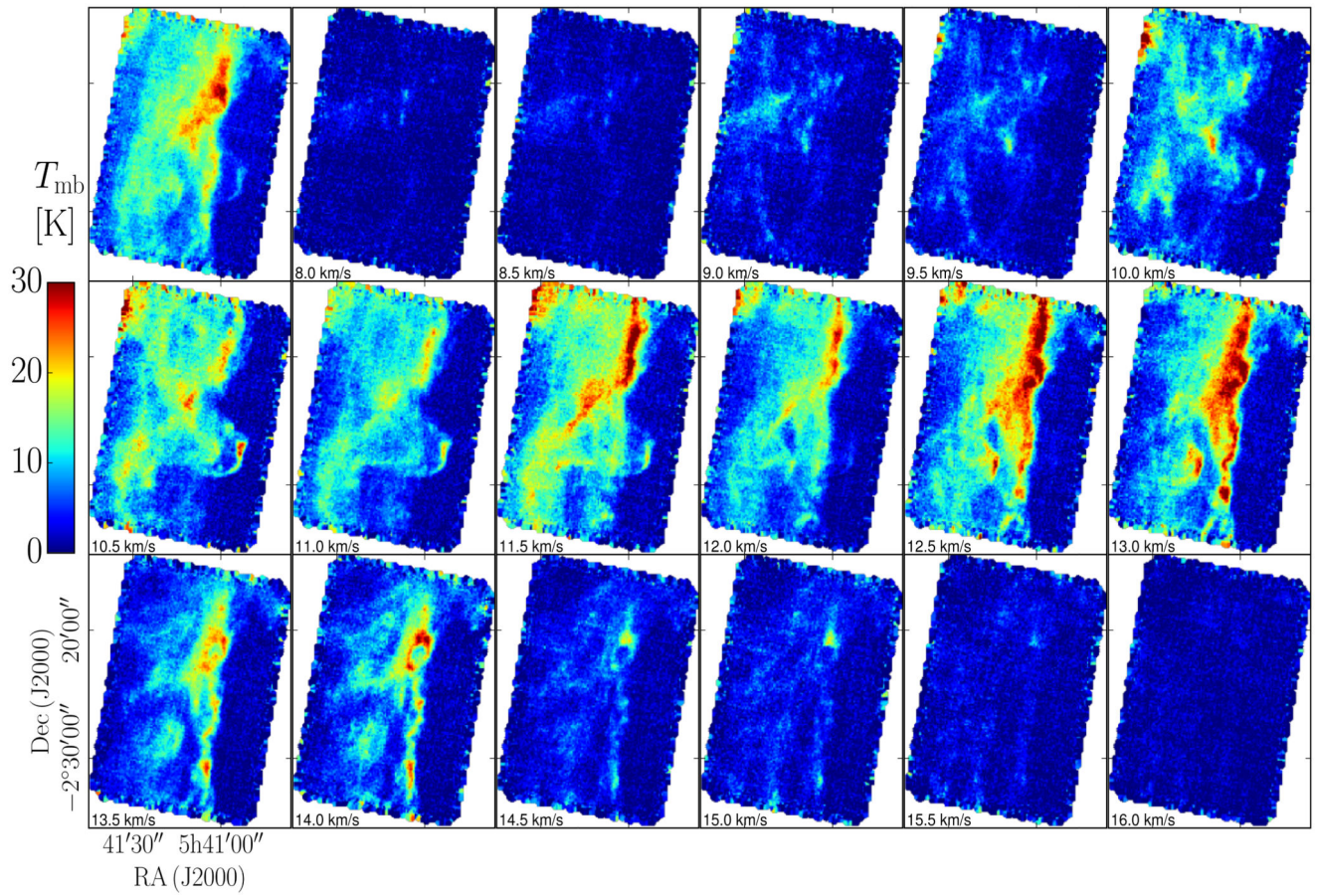
Fig. 4. [Cu II] channel maps from 8.0 \text{ km s}^{-1} to 16.0 \text{ km s}^{-1} in steps of d\nu = 0.5 \text{ km s}^{-1} at 15.9'' resolution. The main-beam temperature T_{\text{mb}} is averaged over the step size d\nu . The first panel shows the line-integrated intensity.
