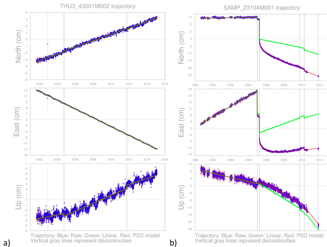
fig.2 a) GNSS position time series at THU3 (Greenland). b) GNSS position time series at SAMP (Indonesia). Source: http://itrf.ign.fr
