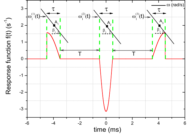
FIG. 11. Response function (in red) of the Mach-Zehnder AI for equal pulses of duration \tau , and considering that the \pi -pulse occurs at t = 0 . Here T = 3 ms and \tau = 1 ms for clarity sake. The intensity of the laser is the same for the first and last laser-pulse (e.g. \Omega_1 = \Omega_3, \Omega_2 = 2\Omega_{1,3} ). The green dash-line symbolises the Raman pulse and the black line represents the Raman frequency ramp characterized with parameters \omega_1^{(i)}, A_i, \beta_i .
