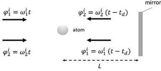
FIG. 10. Scheme of the cold atom interferometer. The resonant counter-propagating beams are obtained by retro-reflecting the lasers on the mirror. Due to the retroreflection delay, if the Raman frequency is not perfectly the same at each Raman pulse, a bias phase arise.
