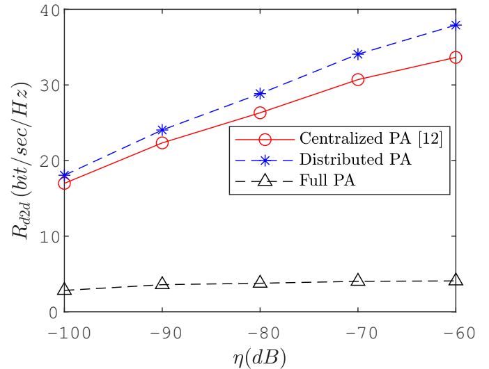
Fig. 4. The achieved D2D rate when allocating power according to: 1) the centralized PA algorithm proposed in [12], 2) the proposed distributed PA algorithm, and 3) the full-power transmission strategy.
