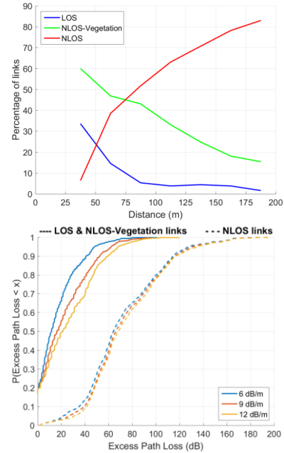
Fig. 7. Distribution of the outdoor propagation results: visibility (left) and Excess Path Loss (right)
