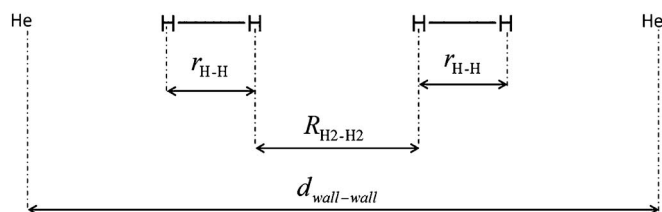
FIG. 10. Two H 2 molecules along a line, surrounded by two helium atoms, the molecular model considered to illustrate the concomitant effect of spatial confinement and orbital interaction.
