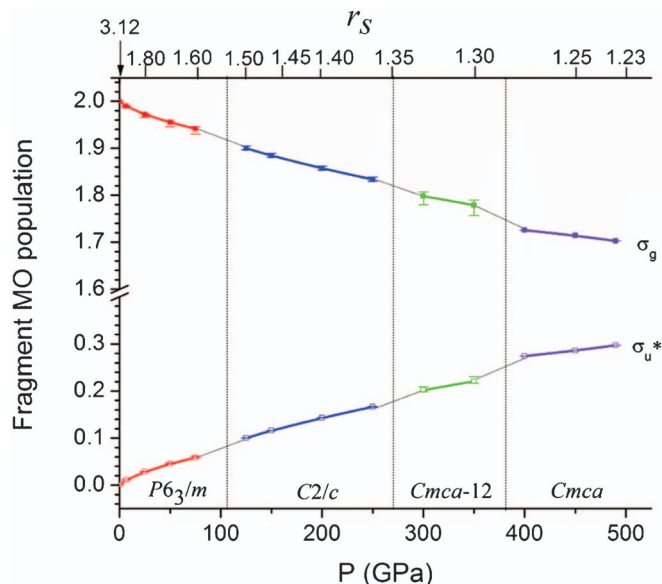
FIG. 4. Population of the fragment \sigma_g and \sigma_u^* MOs in hydrogen as a function of pressure (averaged over the unit cell), as calculated by the extended Hückel method. Recall that at 490 GPa the relative compression is 15.8. The slight “spread bars” show the range of populations found.
