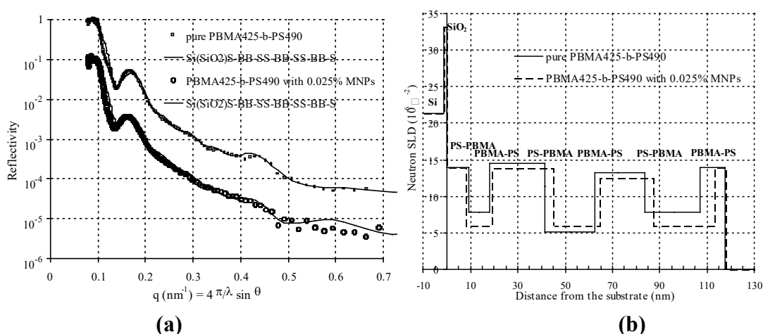
Figure 2: (a) Neutron Reflectivity spectra of a pure copolymer film (squares) and of a copolymer film doped at 0.025% with PS@ \gamma -Fe 2 O 3 magnetic nanoparticles (circles, shifted by a factor 0.1 for the sake of clarity). (b) Calculated scattering length density (SLD) profiles used to fit the neutron reflectivity spectra (solid lines trough experimental data points of curves (a) ).
