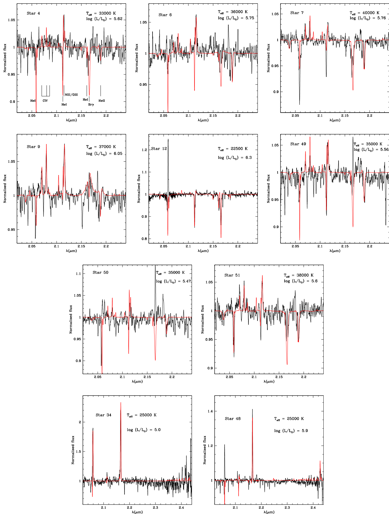
Fig. 4. Best fit (red) of the observed spectrum (black) of stars for which the spectrum quality was sufficient to perform a spectroscopic analysis. The main diagnostic lines are indicated in the upper left panel .
