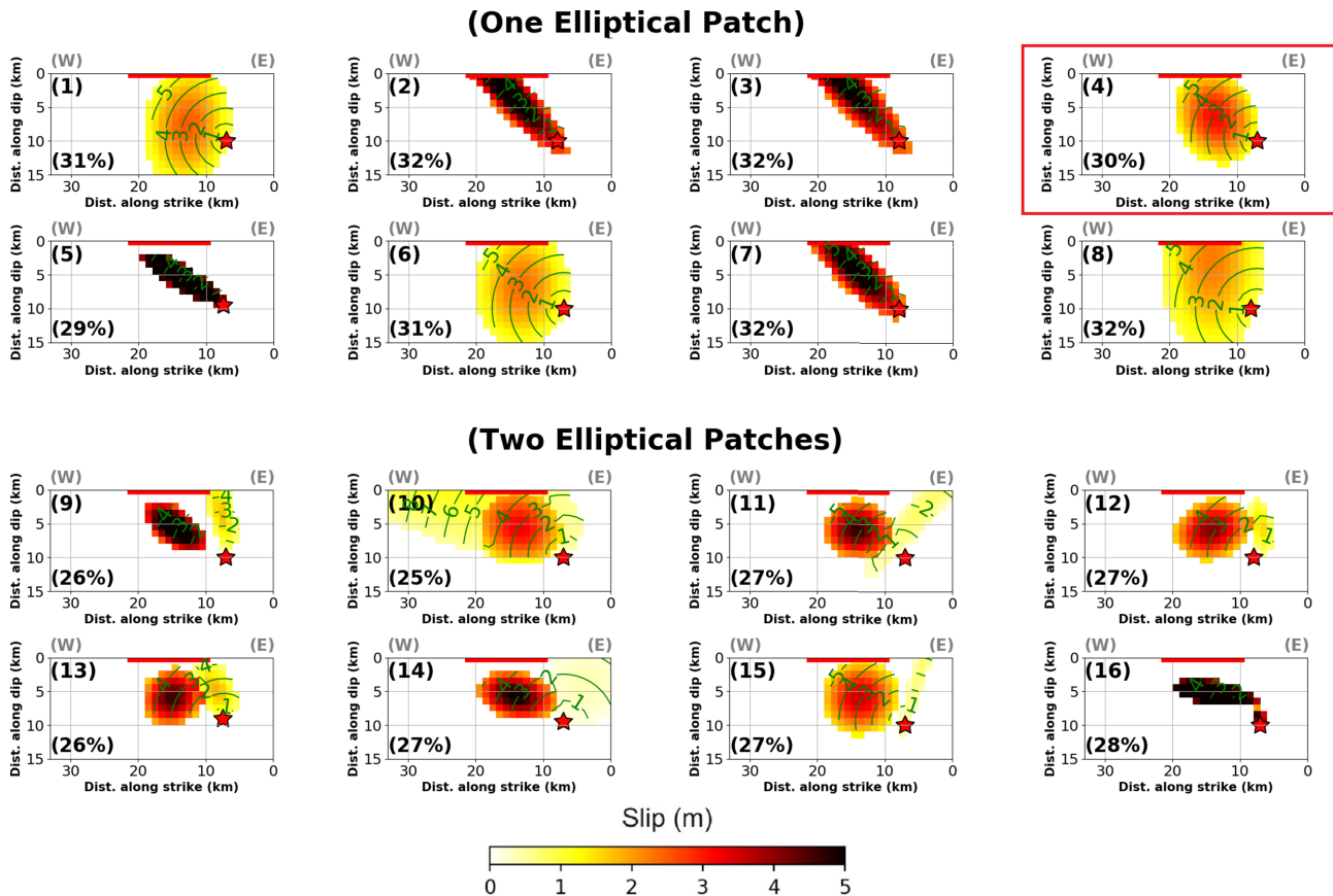
Figure 4. 16 kinematic rupture models of M1 calculated by inverting near-field strong motion displacement time histories on the fault plane with strike/dip of 88^{\circ}/80^{\circ}\text{S} using one and two elliptical slip patches. Each subfigure is labelled with a number on the left top. The fault dimension is in kilometres. The X -axis show distance along strike and Y -axis is along downdip. The misfit of each model is written on the left bottom of each subfigure. The star is the earthquake hypocentre. Curved lines are positions of rupture front in time (seconds) after the origin time. Solid straight lines are positions of the reported surface rupture. The slip is saturated at 5 m. The best model (4) is highlighted by the box.
