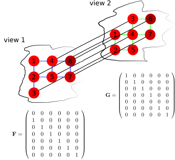
Fig. 5: Example of correspondence functions \mathbf{F} and \mathbf{G} computed for a small shape-varying super-pixel. The graph nodes are labeled in both graphs following a vertical scan line. In the second view, we have one disappearing node and another appearing one with respect to the first view.
