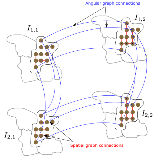
Fig. 3: Example of edges drawn inside a super-ray. We can see the connections within super-pixels in each view (i.e. spatial connections in red), as well as connections between pixels belonging to different views (i.e. angular connections in blue, only a subset of the connections is shown for illustration purpose). The color assigned to the vertices are the color values of the light field.
