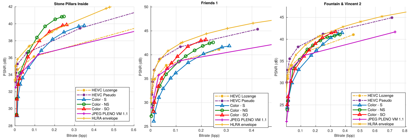
Fig. 12: Rate distortion performance of our graph based coding schemes (Non separable, not optimized and optimized separable graph transforms) compared to HEVC lozenge [1], HEVC pseudo [3], HLRA [4] and JPEG Pleno VM 1.1 [2] for the 9 \times 9 light fields used in the ICIP 2017 Grand Challenge [45] following the common test conditions.
