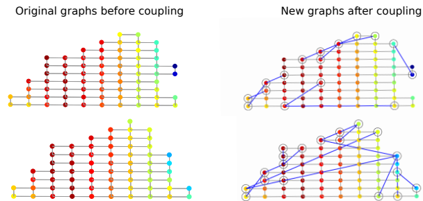
Fig. 10: Image showing the old graphs before coupling and the new graphs after optimization. New edges with absolute weight values larger than 0.04 are shown as blue lines connecting highlighted nodes.
