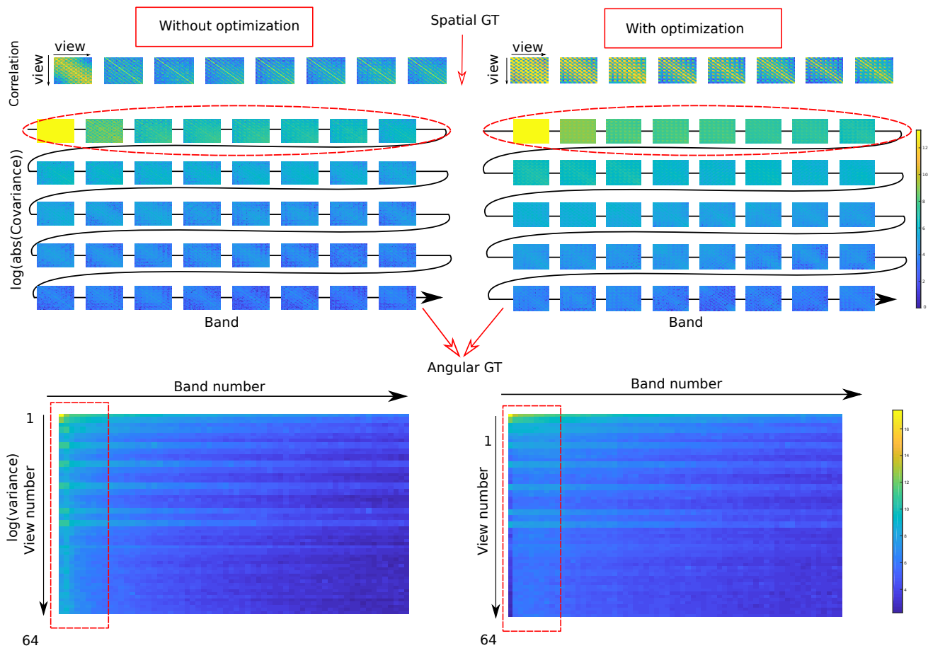
Fig. 11: Advantage of our optimization in terms of energy compaction. The three rows correspond to (1) correlation matrices of the spatial transformed coefficients of the first ten bands, (2) the log of the absolute value of the covariance matrices of the 64 first bands of the spatial transformed coefficients, and (3) the logarithm of the variance of the coefficients after the angular transform, respectively. The two columns show the two cases: without or with our optimization.
