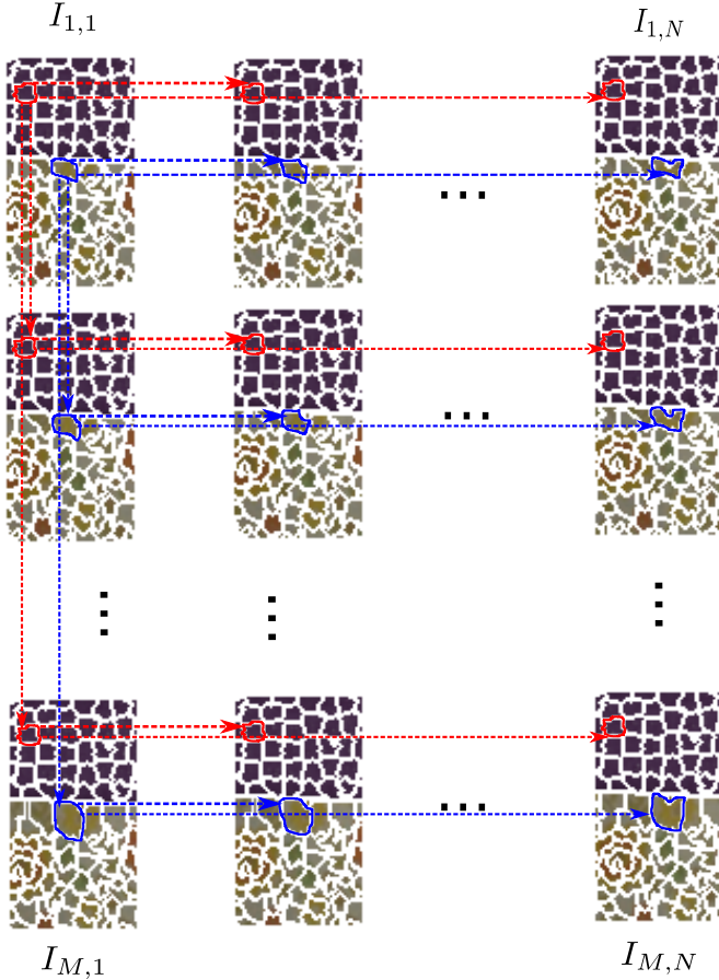
Fig. 2: Image showing the super-ray construction. The algorithm proceeds row by row. In the first row, only horizontal projections are performed. In every other row, first a vertical projection then N - 1 horizontal projections are performed. The red super-pixel in I_{1,1} is consistent across views, whereas the super-pixel in blue is shape-varying.
