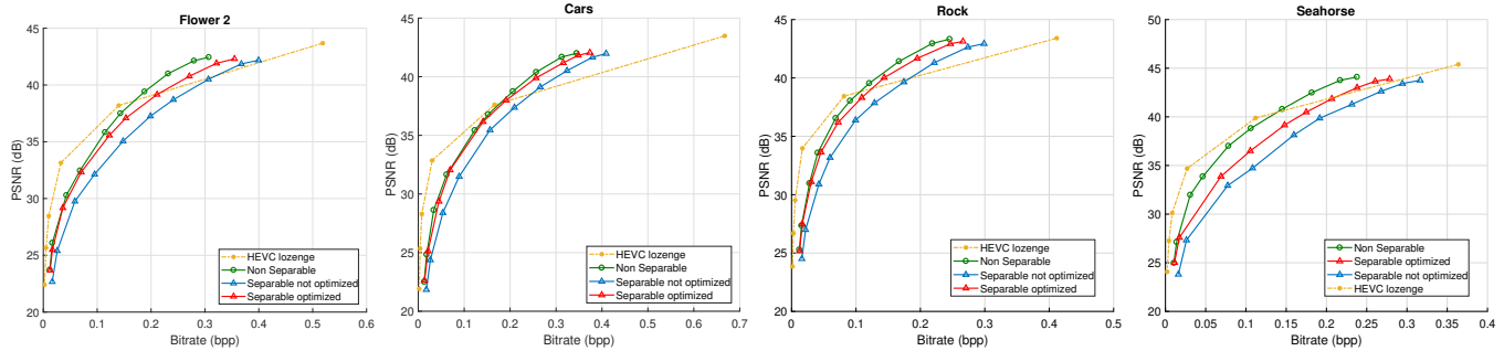
Fig. 13: Rate distortion performance of our graph based coding schemes (Non separable, not optimized and optimized separable graph transforms) compared to HEVC lozenge [1] for the 8 \times 8 light fields of [35].
