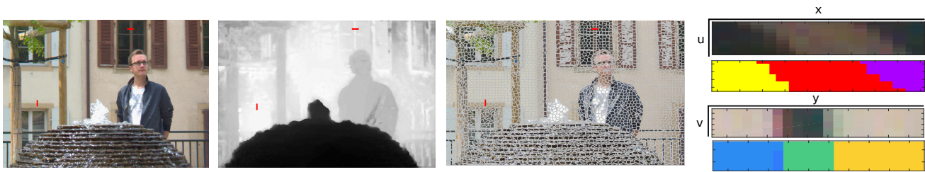
Fig. 1: The result of our proposed light field segmentation for a dense light field Fountain Vincent (from EPFL light fields dataset) with an estimated disparity. From left to right, the original view I_{1,1} , the disparity map of the original view, the super-pixel segmentation of I_{1,1} and an example of vertical and horizontal epipolar segments taken from both original 4D RGB light field and the 4D segmentation labels (The red lines inside the images show from where the epipolar line is extracted).
