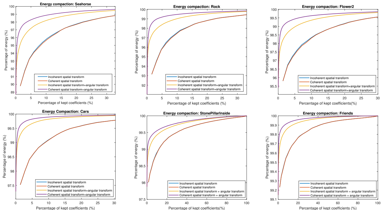
Fig. 9: Energy compaction with or without optimization of the first spatial transform for four datasets (Seahorse, Rock, Flower2 and Cars) from the dataset used in [35] and two others (Friends and StonePillarsInside) taken from the datasets in [45].
