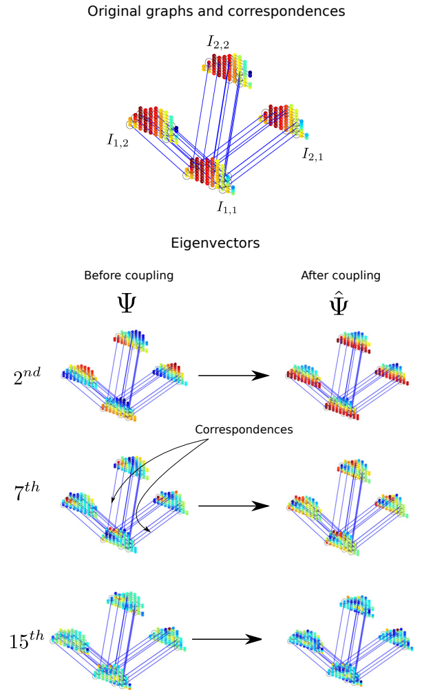
Fig. 8: Illustration of the output of the optimization process for a super-ray in 4 views. The first row corresponds to a super-ray across four views of the light field. The signal on the vertices correspond to the color values lying on super-pixels corresponding to the same super-ray and the blue lines denote the correspondences. The second to fourth rows are illustrations of basis functions before and after optimization. The signals on the vertices are the eigenvectors values.
