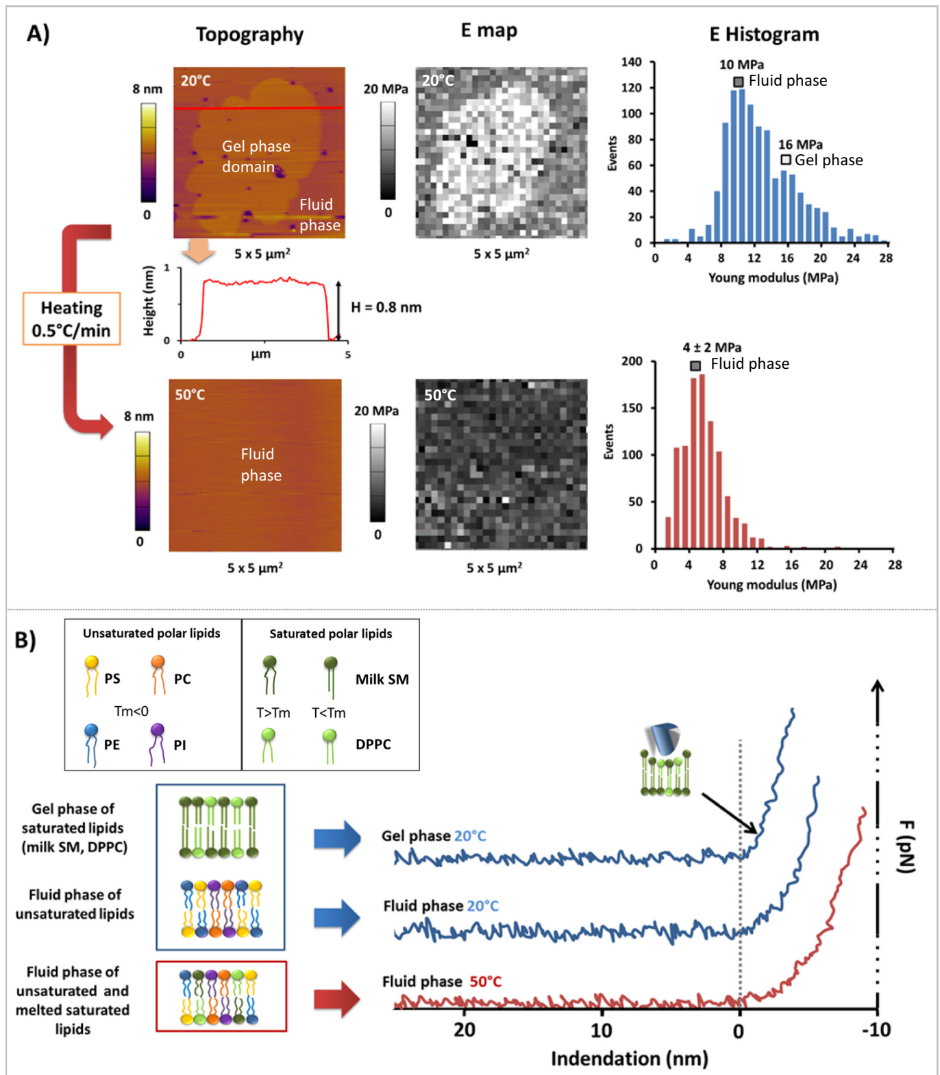
Fig. 3. (A) Effect of heating on the lateral organization and the mechanical properties of MFGM polar lipids supported bilayers investigated by atomic force microscopy (AFM). AFM images and the corresponding Young modulus mapping and histograms were recorded at 20 °C and 50 °C in PIPES-NaCl-CaCl 2 buffer, pH 6.7. (B) Typical force-distance curve recorded onto the gel or fluid phases at 20 °C or onto the fluid phase at 50 °C.
