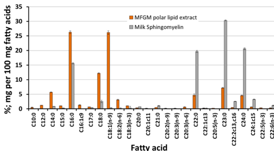
Fig. 1. (A) Composition, in % weight of the total polar lipids, of the milk fat globule membrane (MFGM) extract in polar lipids PE (phosphatidylethanolamine), PI (phosphatidylinositol), PS (phosphatidylserine), PC (phosphatidylcholine) and MSM (milk sphingomyelin); (B) Composition, in % weight, of the fatty acids present in the polar lipids of the MFGM extract (in orange) and in the milk sphingomyelin as a reference (in grey).
