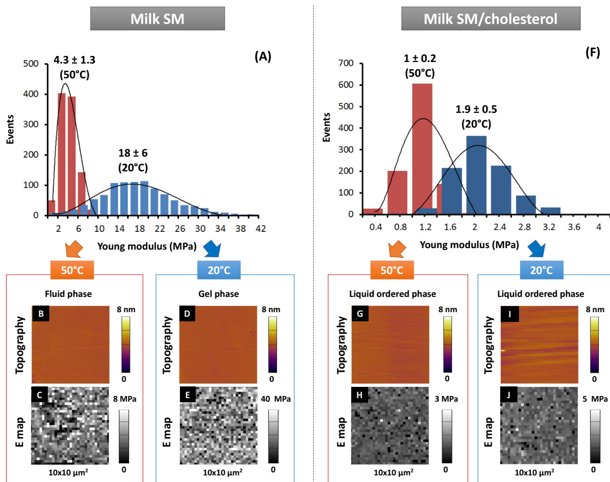
Fig. 4. Effect of the phase state of milk SM, as modified by temperature and cholesterol, on the topography and Young modulus values of supported milk SM bilayers. AFM topography images, Young modulus mapping and the corresponding histograms were recorded at 20\text{ }^{\circ}\text{C} or 50\text{ }^{\circ}\text{C} in PIPES-NaCl-CaCl 2 buffer, pH 6.7.
