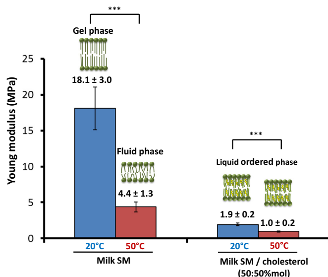
Fig. 5. Comparison of the average Young modulus values obtained at 20\text{ }^{\circ}\text{C} or at 50\text{ }^{\circ}\text{C} in PIPES-NaCl-CaCl 2 buffer, pH 6.7, on indenting milk SM or milk SM/chol (50:50 mol%; liquid ordered phase) supported bilayers. Symbol *** means significant difference ( p < 0.05 ; N = 2-9 images for each category).
