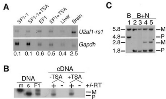
FIG. 3. U2af1-rs1 expression and methylation are unaltered in TSA-treated cells. A , Northern analysis of total RNA samples. Hybridization was with U2af1-rs1 probe 1 (upper panel) and a Gapdh control probe, respectively. The latter yielded the same relative band intensities as a probe hybridizing to 18 S and 28 S RNA (data not shown). U2af1-rs1:Gapdh ratios of band intensities are indicated. B , unaltered paternal U2af1-rs1 expression. The lanes to the left show amplifications from C57BL/6 ( m ), M. spretus ( s ), and (C57BL/6 × M. spretus )F1 ( F1 ) DNAs, respectively. The lanes to the right show expression from cDNA samples corresponding to untreated and TSA-treated SF1-1 ES cells. To exclude possible DNA contamination, we performed parallel assays without the addition of reverse transcriptase (–). C , U2af1-rs1 methylation in EF1 and SF1-1 cells. Bgl II ( B ) and Bgl II + Not I ( B+N )-digested DNA samples were analyzed by Southern hybridization with probe 1. Lanes 1 and 2, (C57BL/6 × M. spretus )F1 liver; lane 3, EF1 fibroblasts; lane 4, SF1-1 ES cells; lane 5, TSA-treated SF1-1 cells. Maternal ( M ) and paternal ( P ) specific fragments are indicated; their sizes are given in kb. The intensity of the 2.8-kb band in lanes 4 and 5 indicates that both in SF1-1 and in TSA-treated SF1-1 cells, ~15% of the maternal chromosomes are not methylated at the Not I restriction site. For the location of the Not I site and probe 1, see Fig. 4A.
