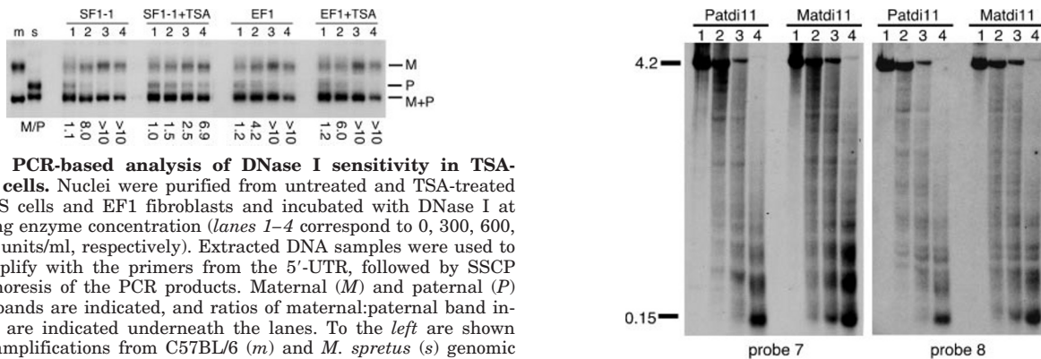
FIG. 4. Southern-based analysis of DNase I sensitivity in TSA-treated cells. A, map depicting the strategy used to analyze parental allele-specific DNase I sensitivity along U2af1-rs1 . Bgl II ( B ), Sac I ( Sa ), and Not I ( N ) restriction sites and probe 1 are indicated. C57BL/6 ( m )- and M. spretus ( s )-specific Bgl II + Sac I fragments are shown underneath. We submitted the nucleotide sequence of this region to GenBank™ (accession number AF309654). B, DNase I assay on (C57BL/6 × M. spretus )F1 kidney cells. After purification, nuclei were incubated at increasing concentrations of DNase I (lanes 1–8 correspond to 0, 50, 100, 200, 300, 400, 500, and 750 units of DNase I/ml, respectively). DNA was extracted subsequently and digested with Bgl II + Sac I, followed by Southern hybridization with probe 1. The 2.5-kb, M. musculus -specific (maternal, M ) and the 1.5-kb, M. spretus -specific (paternal, P ) bands are indicated. Measured maternal:paternal ( M/P ) ratios of band intensities are indicated underneath the lanes; –, bands are too weak to determine M/P ratios. The three lanes to the left show Bgl II + Sac I-digested genomic DNAs from C57BL/6 ( m ), M. spretus ( s ), and (C57BL/6 × M. spretus )F1 ( F1 ) DNAs, respectively. C, DNase I assay on ES cells. Nuclei from untreated and TSA-treated SF1-1 cells were incubated at increasing concentrations of DNase I (lanes 1–7 correspond to 0, 50, 100, 200, 300, 400, and 500 units of DNase I/ml, respectively). Southern hybridization with probe 1 was the same as in B. Maternal:paternal ratios are indicated underneath the lanes. D, DNase I assay on EF1 fibroblasts. Lanes 1–7 correspond to 0, 100, 200, 300, 400, 500, and 750 units/ml, respectively. Southern hybridization with probe 1 was the same as in B.
