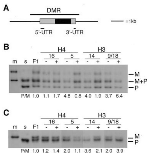
FIG. 2. In ES cells, TSA alters acetylation of H4-lysine 5 and H3-lysine 14 acetylation along U2af1-rs1 . A, map of the U2af1-rs1 gene, shown as a box with its coding part in black. The line above represents the domain of maternal DNA methylation and differential generalized DNase I sensitivity (10). Small bars indicate the regions analyzed by PCR-SSCP. B, acetylation at the 5'-UTR of U2af1-rs1 . ChIP was performed simultaneously on nontreated (-) and TSA-treated (+) SF1-1 ES cells, and PCR on the corresponding DNA samples was with primers from the 5'-UTR. The first three lanes show PCR products (after SSCP electrophoresis) from control liver DNAs of C57BL/6 (m), M. spretus (s), and (C57BL/6 × M. spretus )F1 (F1), respectively. Subsequent lanes show PCR amplifications following ChIP with antisera to H4Ac16, H4Ac5, H3Ac14, and H3Ac9/18, respectively. Maternal (M) and paternal (P) allele-specific fragments are indicated. C, acetylation at the 3'-UTR of U2af1-rs1 . Amplification from the same DNAs was with primers from the 3'-UTR.
