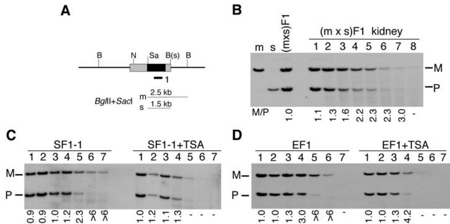
FIG. 4. Southern-based analysis of DNase I sensitivity in TSA-treated cells. A, map depicting the strategy used to analyze parental allele-specific DNase I sensitivity along U2af1-rs1 . Bgl II ( B ), Sac I ( Sa ), and Not I ( N ) restriction sites and probe 1 are indicated. C57BL/6 ( m )- and M. spretus ( s )-specific Bgl II + Sac I fragments are shown underneath. We submitted the nucleotide sequence of this region to GenBank™ (accession number AF309654). B, DNase I assay on (C57BL/6 × M. spretus )F1 kidney cells. After purification, nuclei were incubated at increasing concentrations of DNase I (lanes 1–8 correspond to 0, 50, 100, 200, 300, 400, 500, and 750 units of DNase I/ml, respectively). DNA was extracted subsequently and digested with Bgl II + Sac I, followed by Southern hybridization with probe 1. The 2.5-kb, M. musculus -specific (maternal, M ) and the 1.5-kb, M. spretus -specific (paternal, P ) bands are indicated. Measured maternal:paternal ( M/P ) ratios of band intensities are indicated underneath the lanes; –, bands are too weak to determine M/P ratios. The three lanes to the left show Bgl II + Sac I-digested genomic DNAs from C57BL/6 ( m ), M. spretus ( s ), and (C57BL/6 × M. spretus )F1 ( F1 ) DNAs, respectively. C, DNase I assay on ES cells. Nuclei from untreated and TSA-treated SF1-1 cells were incubated at increasing concentrations of DNase I (lanes 1–7 correspond to 0, 50, 100, 200, 300, 400, and 500 units of DNase I/ml, respectively). Southern hybridization with probe 1 was the same as in B. Maternal:paternal ratios are indicated underneath the lanes. D, DNase I assay on EF1 fibroblasts. Lanes 1–7 correspond to 0, 100, 200, 300, 400, 500, and 750 units/ml, respectively. Southern hybridization with probe 1 was the same as in B.
