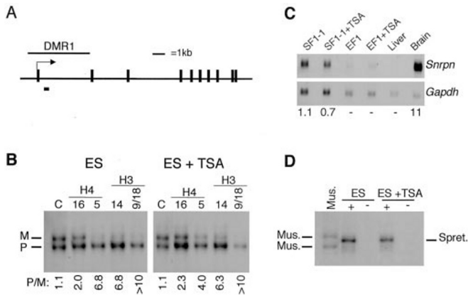
FIG. 7. Allelic acetylation at DMR1 of Snrpn is unaltered by TSA. A , map of the Snrpn gene, with exons 1–10 (filled boxes) and the differentially methylated region comprising exon 1 (DMR1, horizontal bar) as defined by Shemer et al. (26). The small bar below indicates the sequences analyzed by PCR-SSCP. B , acetylation of Snrpn in untreated (ES) and TSA-treated (TSA+TSA) ES cells. PCR-SSCP was performed on the same ChIP assays as described in the legend to Fig. 2 B , and amplification was with primers from the DMR1 of Snrpn . Lanes C correspond to amplification from input chromatin without the addition of antiserum. C , Snrpn expression in TSA-treated ES cells. Northern blot hybridization was with an Snrpn , exon 7 (upper panel) and a Gapdh probe, respectively. Snrpn:Gapdh ratios of band intensities are indicated. This yielded the same relative intensities as compared with a probe hybridizing to 18 S and 28 S RNA (data not shown). D , unaltered paternal Snrpn expression. The lane to the left shows amplification (201-bp fragment covering exons 1–3) from C57BL/6 cDNA (from liver). To the right, amplification from cDNA samples corresponding to untreated (ES) and TSA-treated (ES+TSA) SF1-1 cells is shown; parallel assays were performed without the addition of reverse transcriptase (–). After denaturation, Mus musculus ( Mus. –) and M. spretus ( Spret. )–specific amplification products were separated by SSCP electrophoresis.
