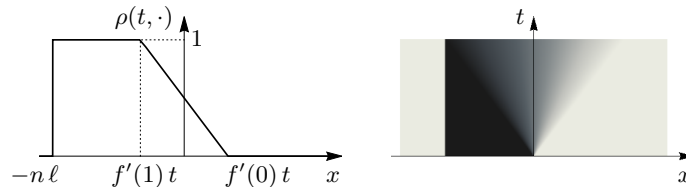
Fig. 3. Solution (18) for t \in (0, -n\ell/f'(1)) . On the right, darker (x, t) -regions correspond to higher densities.
