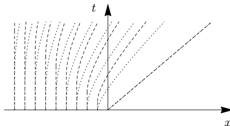
Fig. 4. Comparison of microscopic (15) (dotted) and macroscopic (19) (dashed) trajectories.
