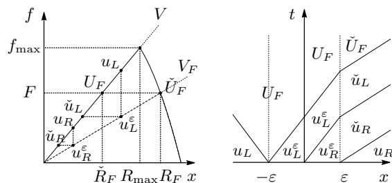
Fig. 6. The approximate solution constructed in Example 3.
