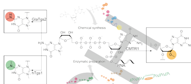
Scheme 1. Schematic representation of 5'-cap methylation by the means of different methyltransferases. RNA equipped with a cap0 structure, prepared either chemically or enzymatically, can be further methylated by cap-modifying methyltransferases. The N 2 -methyltransferases GlaTgs2 and hTgs1 convert the N 2 -methyl guanosine into the di- or tri-methyl mRNA caps 2 m,7m Gppp or 2 m,2m,7m Gppp, respectively. The first transcribed nucleotide can be methylated at its 2'-position by the human 2'-O-methyltransferase CMTR1.
