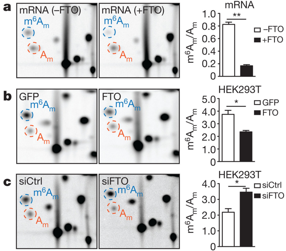
Figure 2. m^6A_m is the preferred substrate of FTO in vivo a , FTO readily demethylates m^6A_m in mRNA. Relative abundance of modified adenosines in mRNA caps derived from mRNA treated with FTO (1 \mu M, 1 h; representative images shown; n = 3 biological replicates; mean \pm s.e.m.; unpaired Student's t -test, **P < 0.001 ). b , FTO expression decreases m^6A_m in HEK293T cells. Relative abundance of modified adenosines in mRNA caps of HEK293T cells expressing GFP (Flag-GFP) or wild-type FTO (Flag-FTO) (representative images shown; n = 3 biological replicates; mean \pm s.e.m.; unpaired Student's t -test, *P < 0.05 ). c , FTO knockdown increases m^6A_m in HEK293T cells. Relative abundance of modified adenosines in mRNA caps of HEK293T cells transfected with scrambled siRNA (siCtrl) or siRNA directed against FTO (siFTO) (representative images shown; n = 3 biological replicates; mean \pm s.e.m.; unpaired Student's t -test, *P < 0.05 ).
