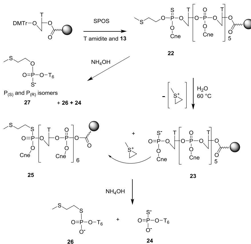
Scheme 4: 5'-thiophosphate-oligonucleotide.
