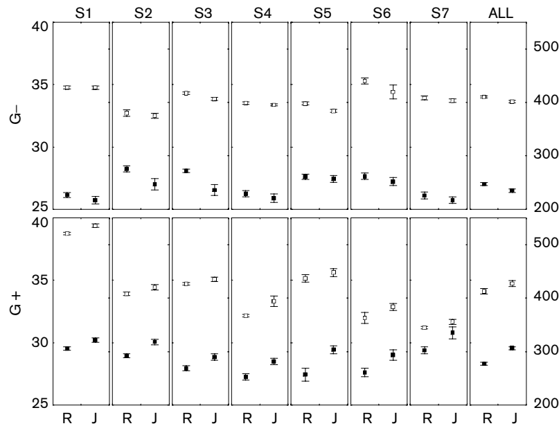
Fig. 1. Mean ( \pm s.e.) amplitude of primary saccade (black squares) and peak velocity (white squares) for each subject (S1–S7) and group (ALL) for the two paradigms (G– and G+).
