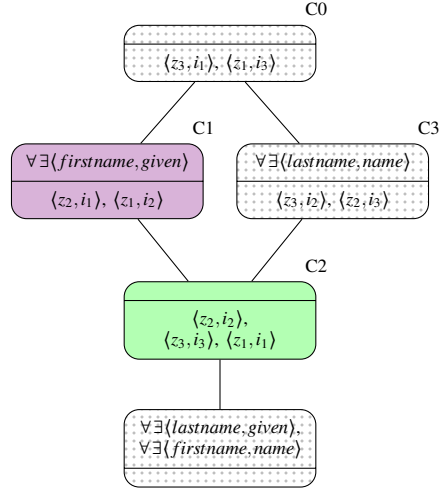
Figure 6: Formal context and concept lattice for Person and Inhabitant of Figure 5.
