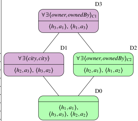
Figure 7: Dependent formal context and concept lattice for House and Place of Figure 5.
