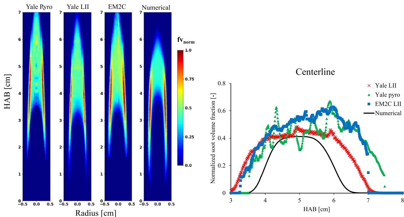
Fig. 6. ISF-coflow-laminar-3 F80: comparison of normalized soot volume fraction in the whole flame cross-section (left) and the along centerline (right) between measurements [81,85,86] and simulation.
