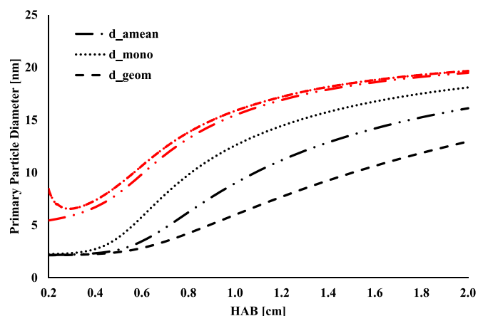
Fig. 2. Simulated d_{\text{amean}} , d_{\text{mono}} and d_{\text{geom}} for two values of the low cut-off size ( d_{pp,N_{\text{min}}} = 2 nm in black and d_{pp,N_{\text{min}}} = 5 nm in red) for the ISF-premixed-laminar-3 flame. (For interpretation of the references to color in this figure legend, the reader is referred to the web version of this article.)
